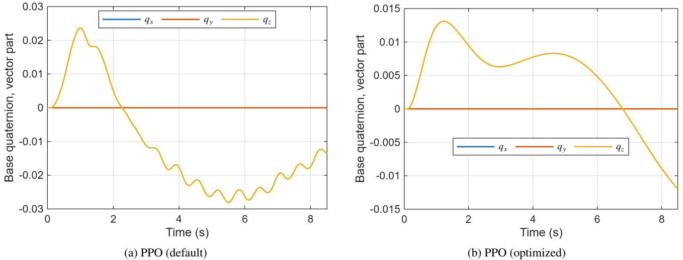
FIGURE 16: [R2.3, A9] Vector part of the base orientation quaternion during the episodes of Fig. 15. The base rotates only about the z -axis. The scalar part stays above 0.9996 in both episodes.
