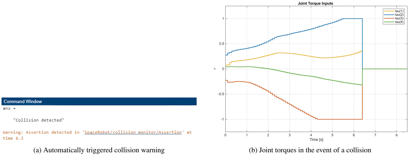
FIGURE 9: Test of the collision monitor and the associated joint torques.
