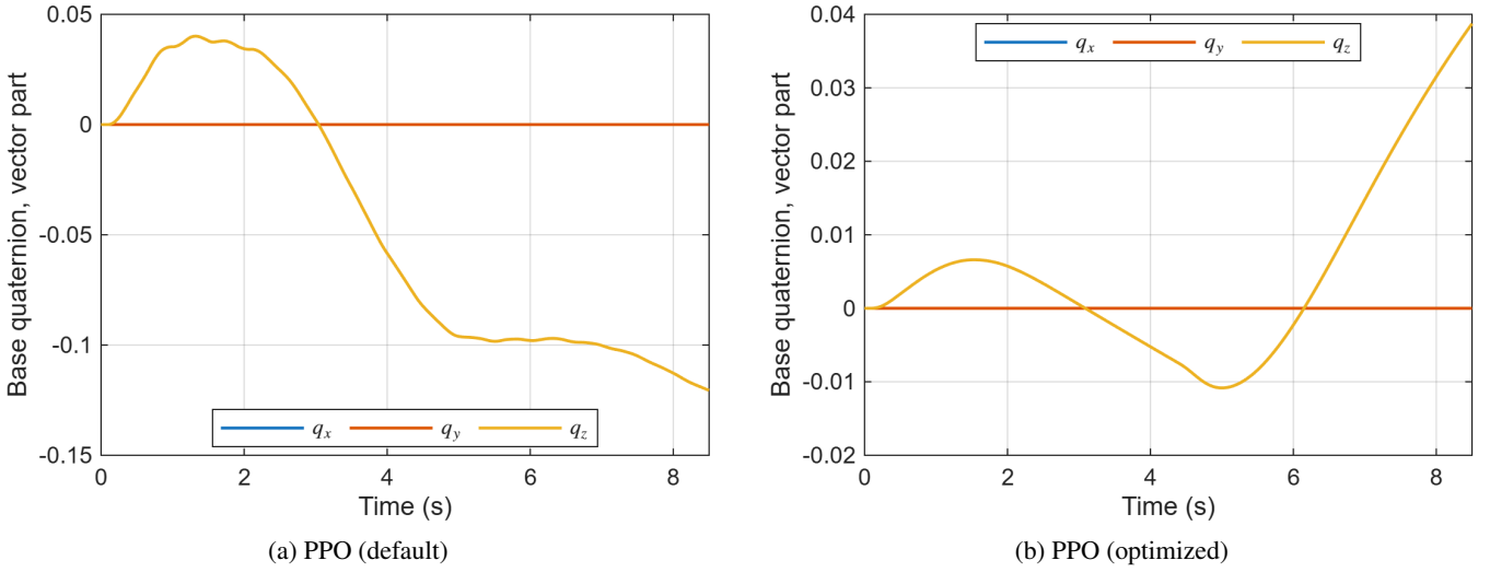
FIGURE 18: [R2.3] Vector part of the base orientation quaternion during the episodes of Fig. 17. The base rotates only about the z -axis. The scalar part stays above 0.992 for the default and above 0.999 for the optimized agent.
