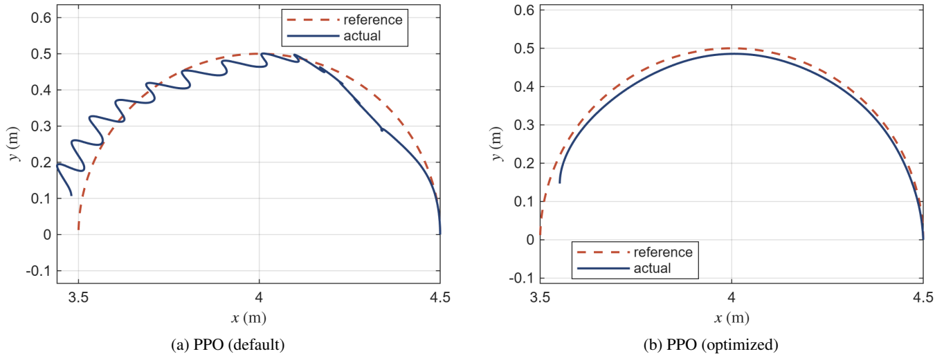
FIGURE 15: [R2.3, A9] Reference and actual end-effector path in the XY plane for one evaluation episode from the nominal initial state. Each panel shows the successful run with the median K_2 of its configuration, seed 2 for the default and seed 0 for the optimized PPO agent.
