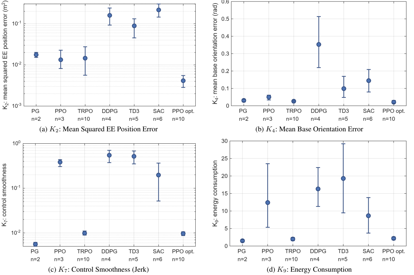
FIGURE 13: [R2.3, A9] Mean and 95% bootstrap confidence interval of selected KPIs over the successful runs of each agent (2000 resamples). The number of successful runs is given below each agent. The intervals of agents with few successful runs are wide or undefined. The optimized PPO agent of Section VII is included for reference.
