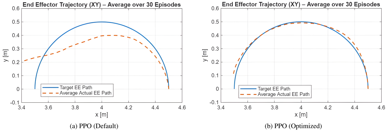
FIGURE 15: Target/actual comparison of the end-effector trajectory in the XY plane.
