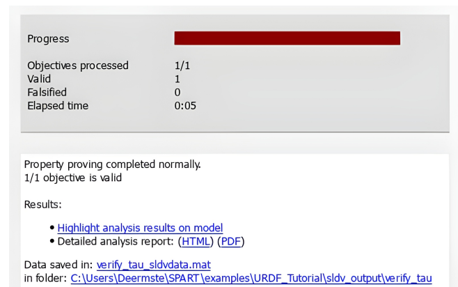
FIGURE 11: Result of the Simulink Design Verifier for the torque-bound property. The analysis found no counterexample for any analyzed execution path [R2.1] of the simplified verification model. The result does not cover other properties or the full nonlinear Simscape model.
