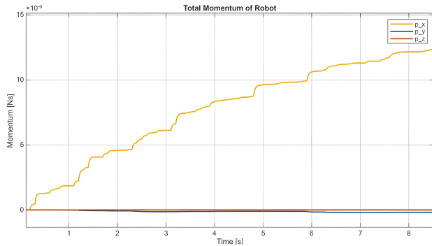
FIGURE 7: Total linear momentum of the robot during an episode.
