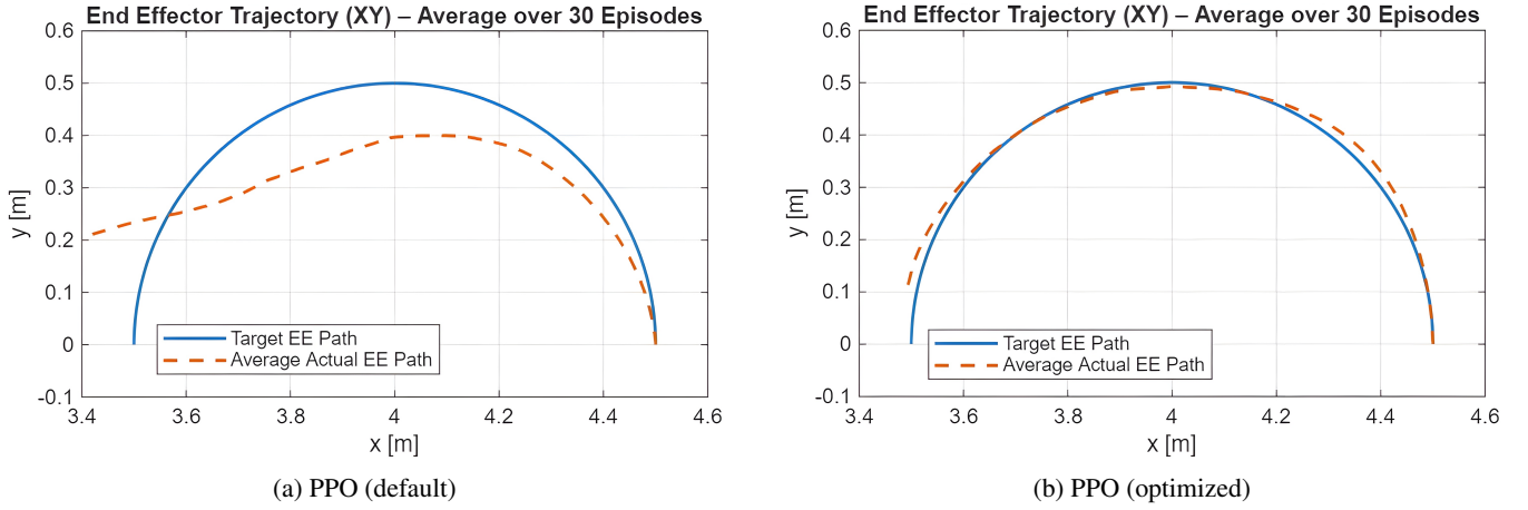
FIGURE 15: Reference and actual end-effector trajectory in the XY plane.
