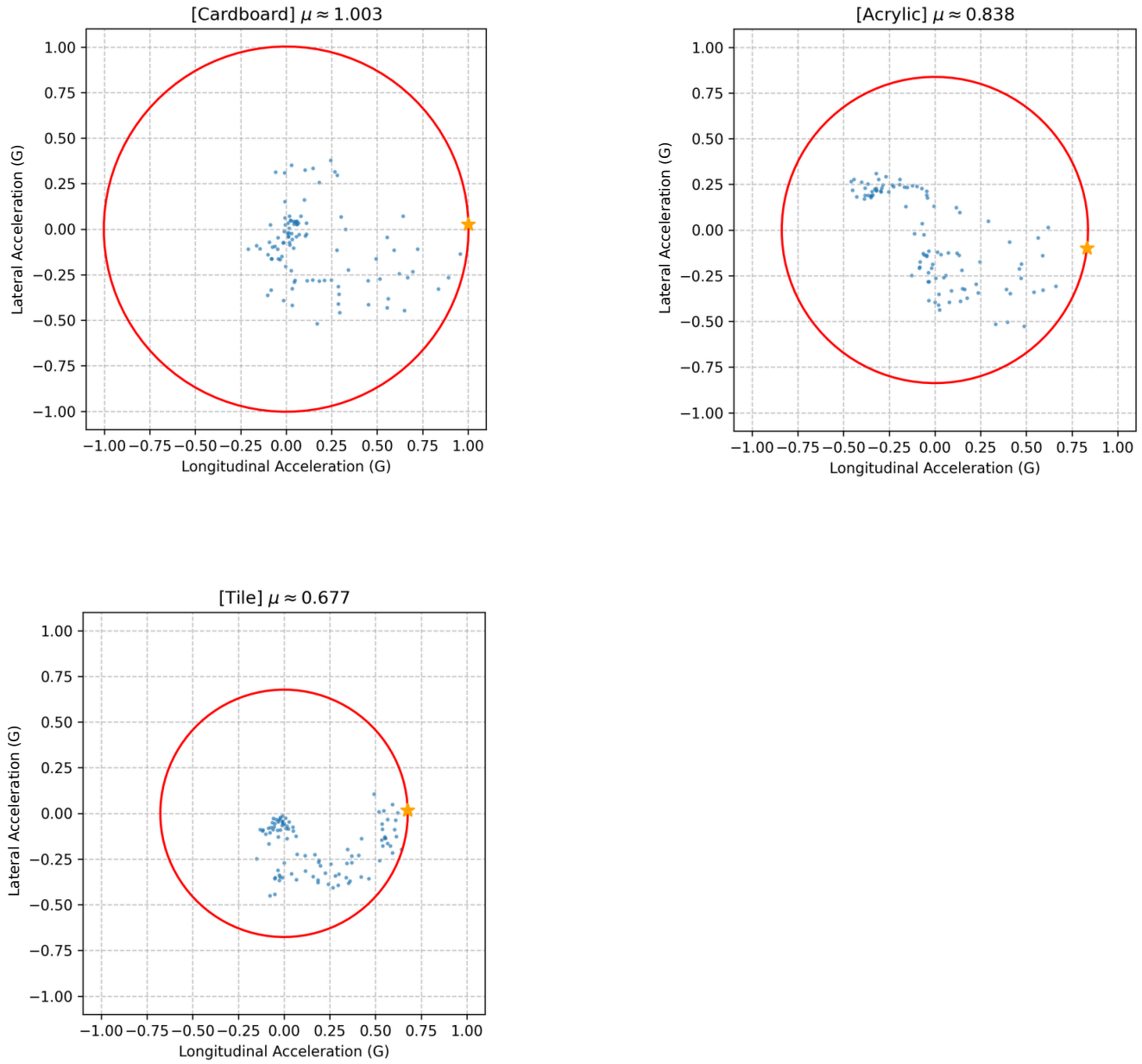
Fig. 1: Friction circle for cardboard, acrylic, and tile. Blue dots denote measured longitudinal and lateral accelerations (in g).
