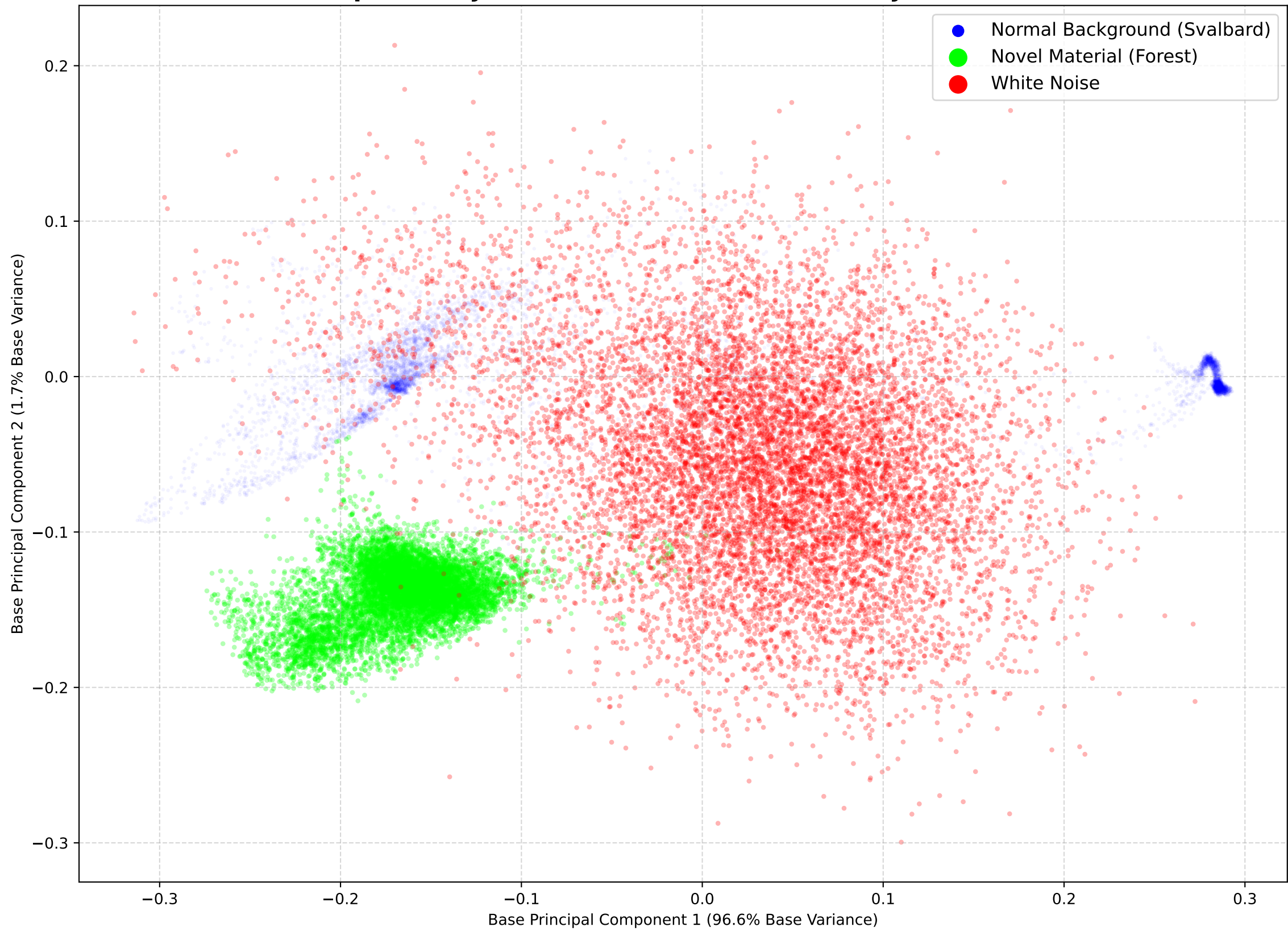
Latent Space Projection: Normal Manifold vs. Injected Anomalies
