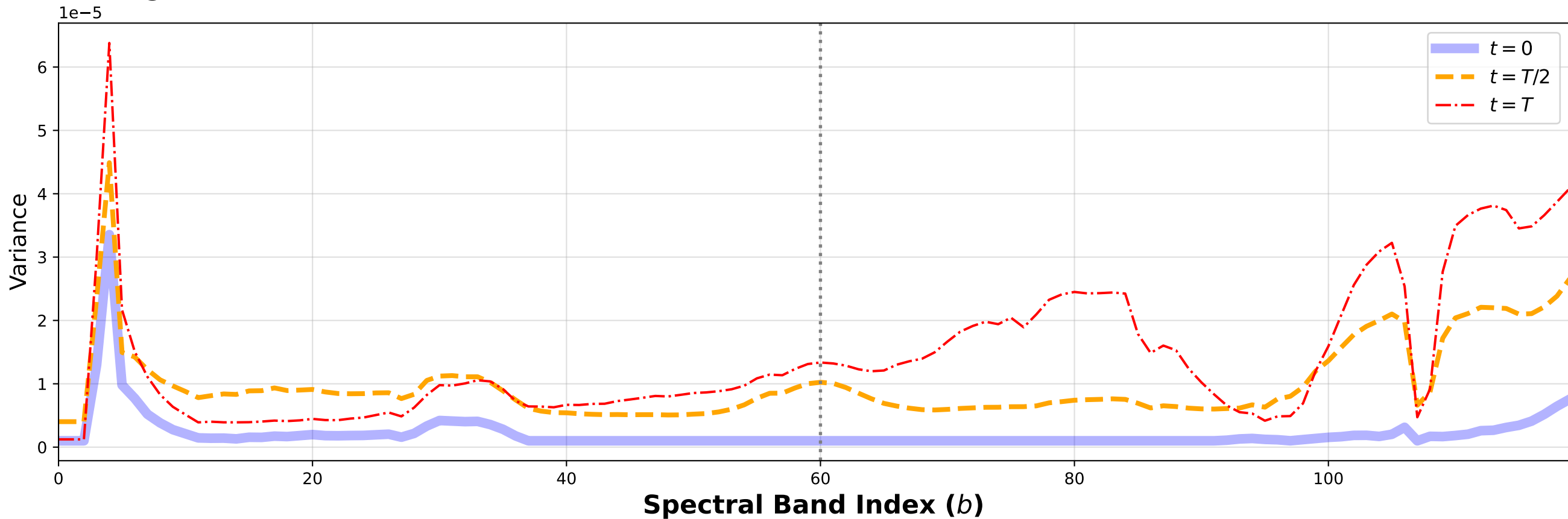
B. Diagonal Noise Variance ( \Psi )
