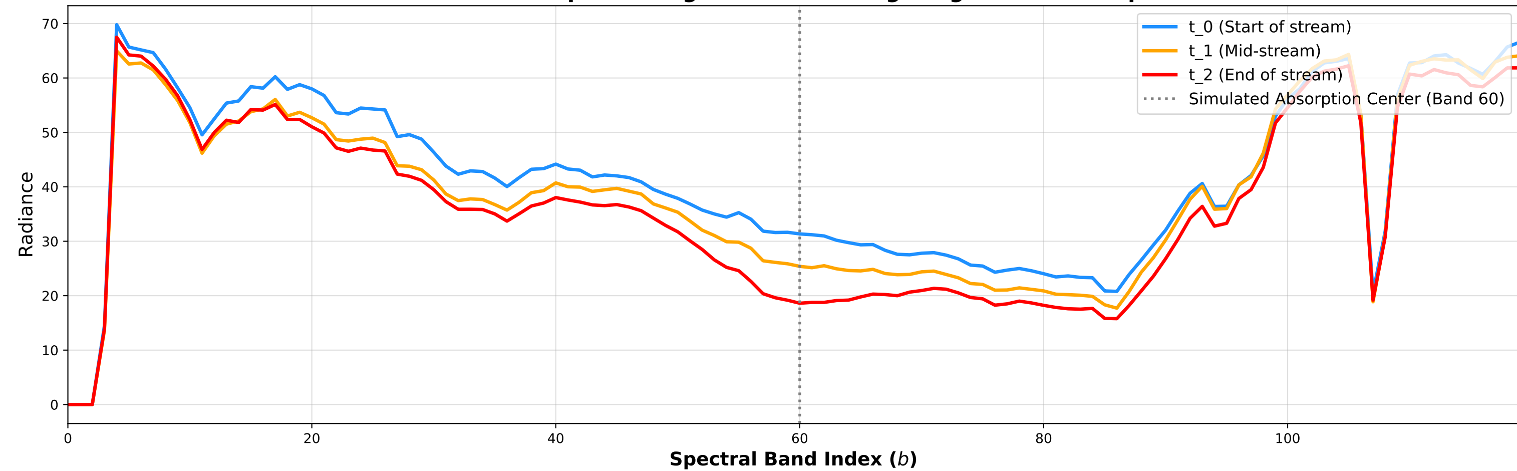
B. Extracted Spectral Signatures Showing Progressive Absorption
