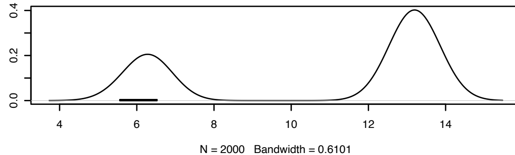
Density of mstar
