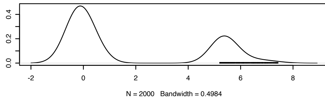
Density of alpha
