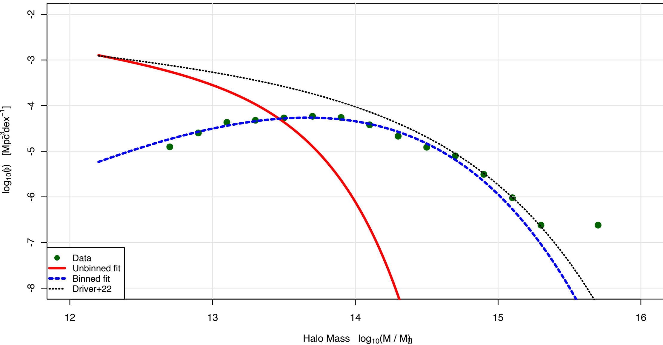
Unbinned vs Binned Fit Comparison
