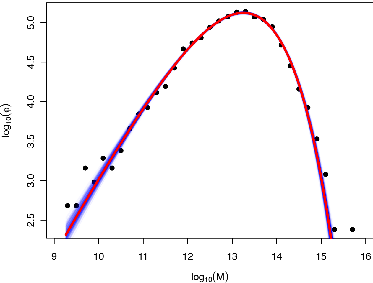
Unbinned MRP Fit
