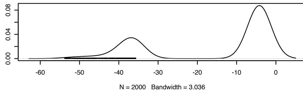
Density of log_phi
