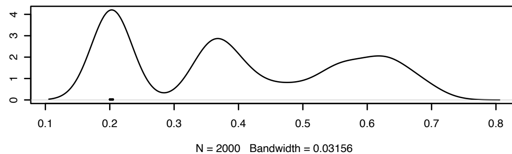
Density of beta
