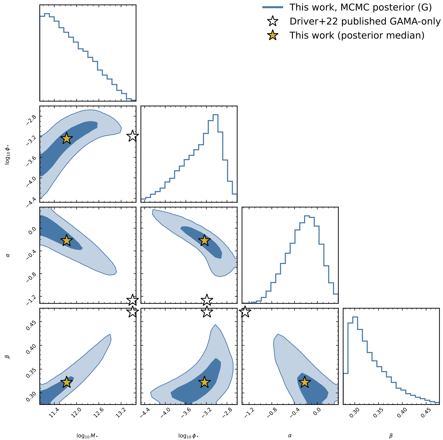
G: MRP posterior, this work
