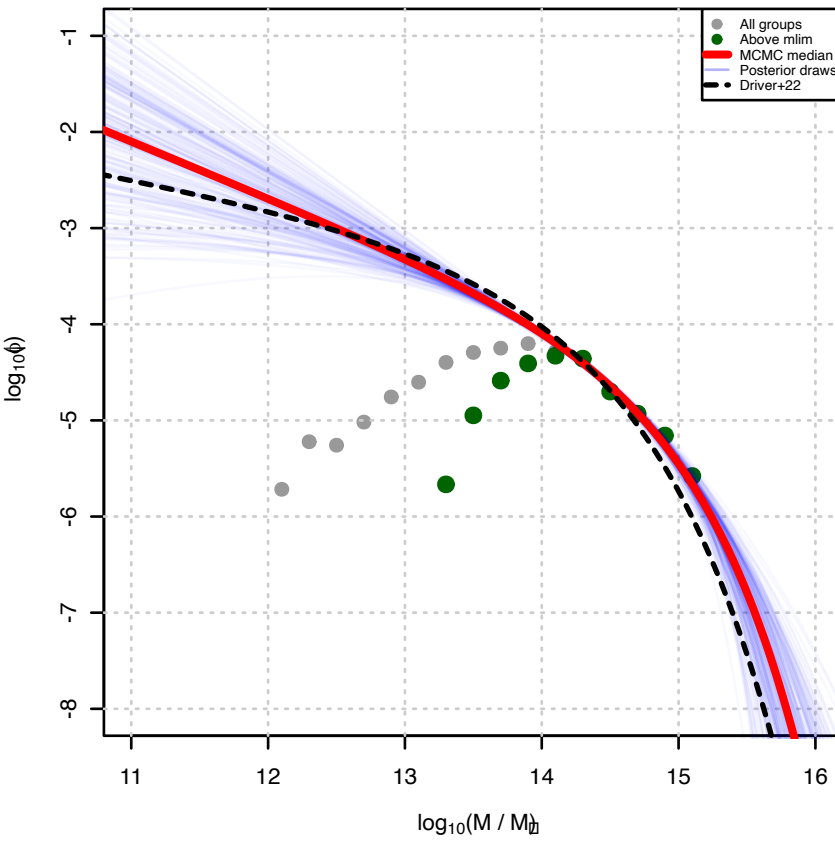
MRP Fit to GAMA
