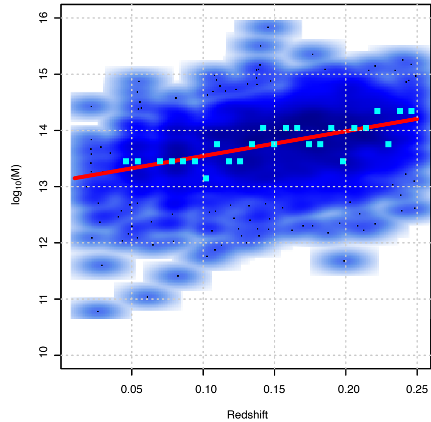
Mass-redshift + mlim(z)
