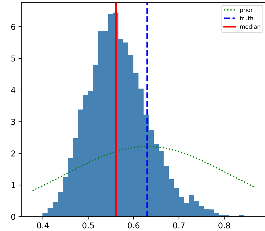
\beta
