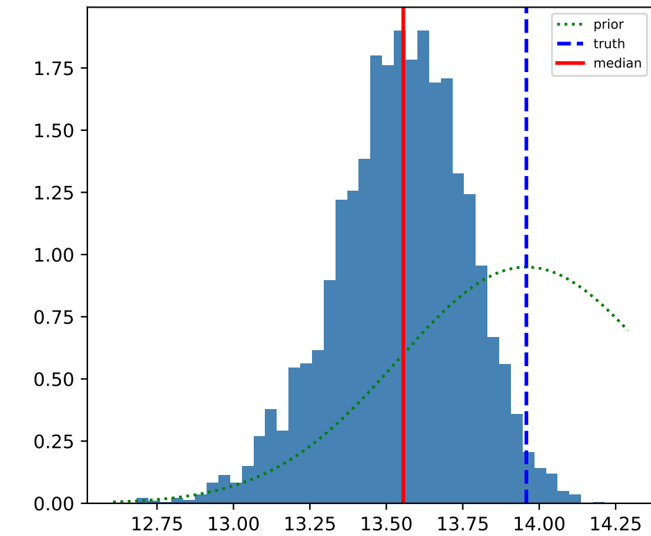
M_*
