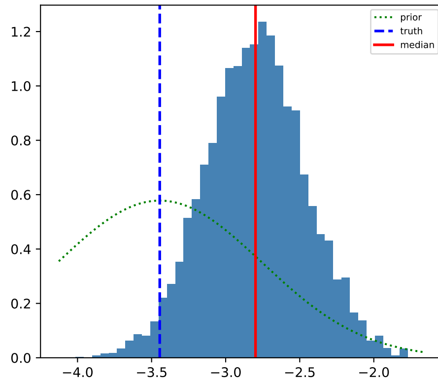
\log \phi_*
