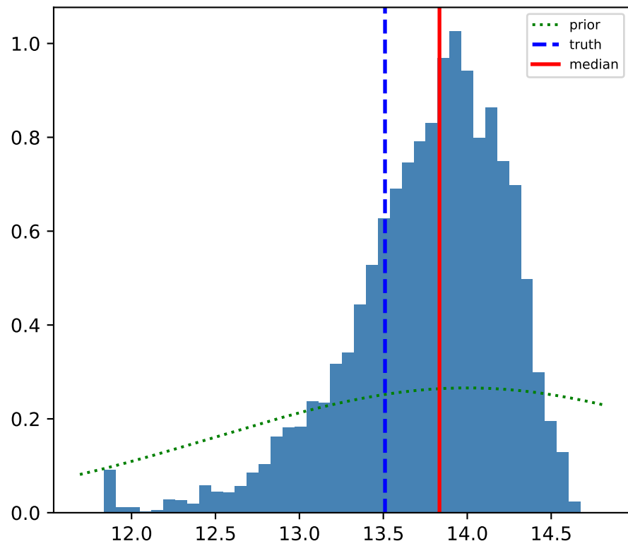
M_*
