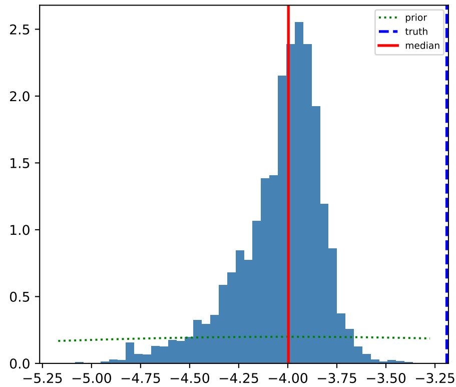
\log \phi_*
