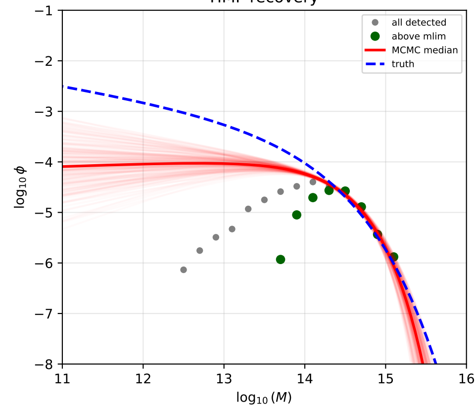
M_*
