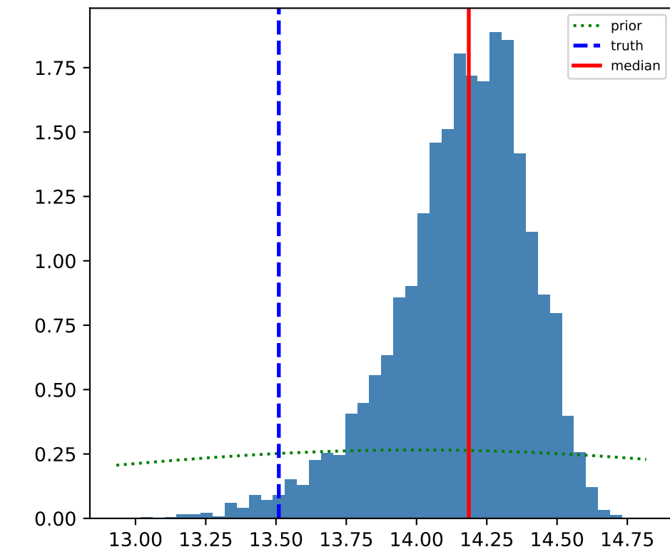
M_*
