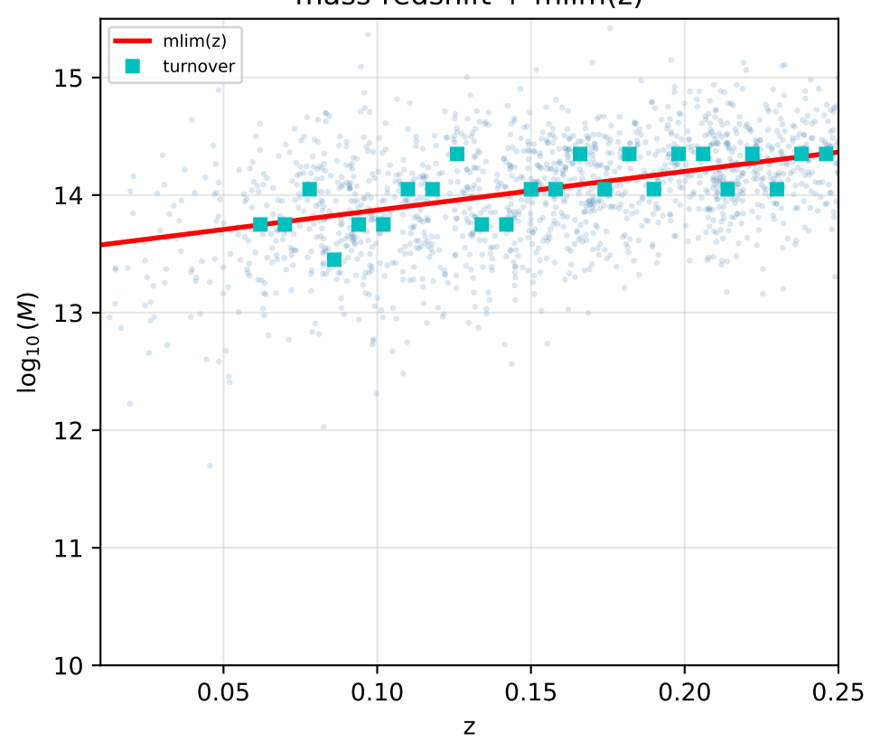
\log \phi_*
