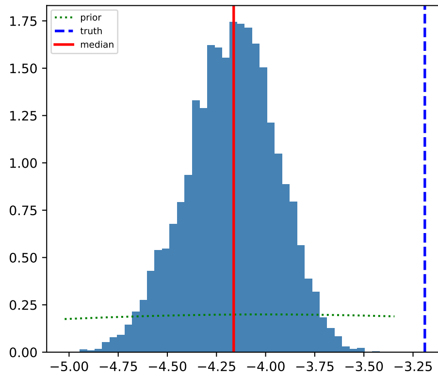
\log \phi_*
