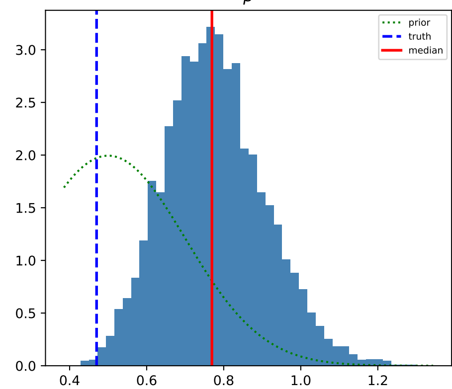
\beta
