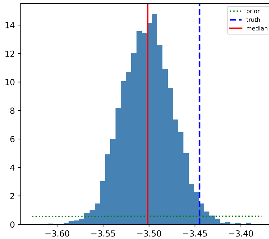
\log \phi_*
