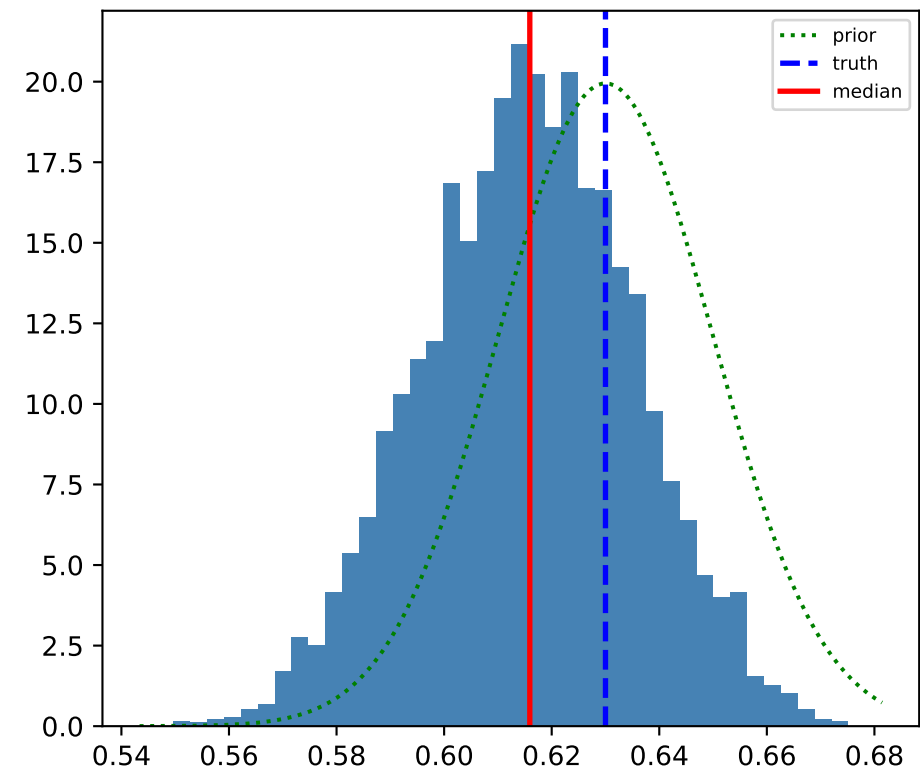
\beta
