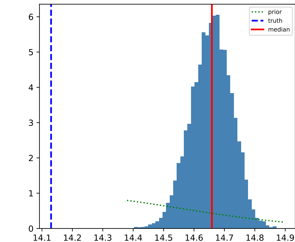
M_*
