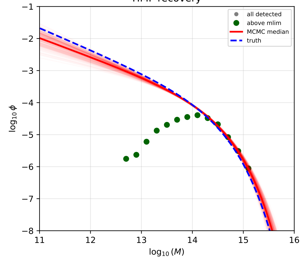
M_*
