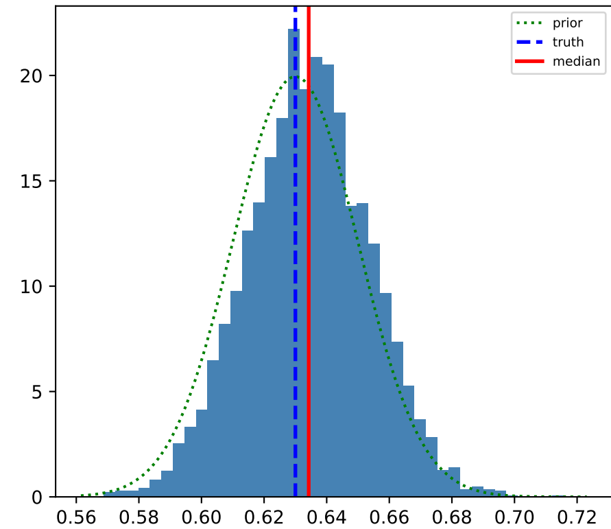
\beta
