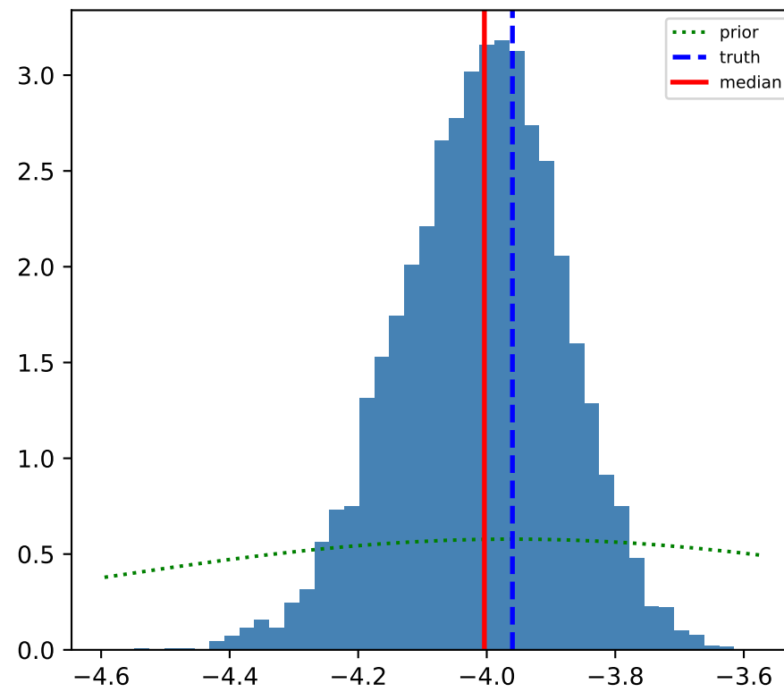
\log \phi_*
