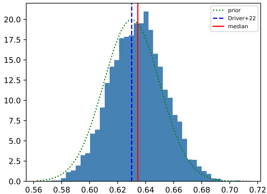
\beta
