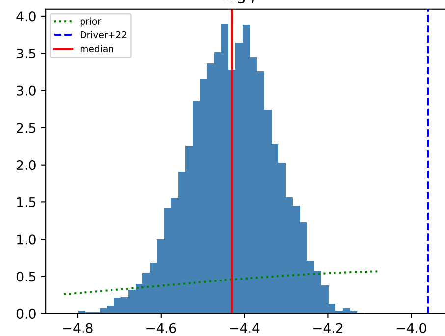
\log \phi_*
