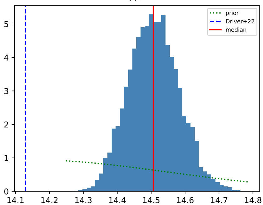
M_*
