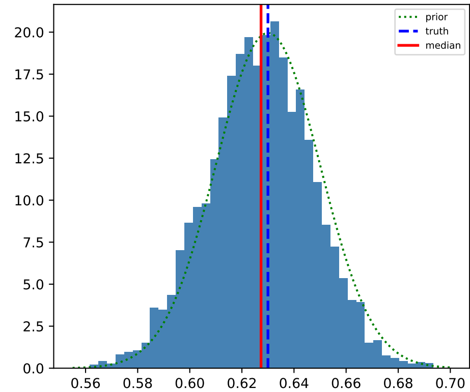
\beta
