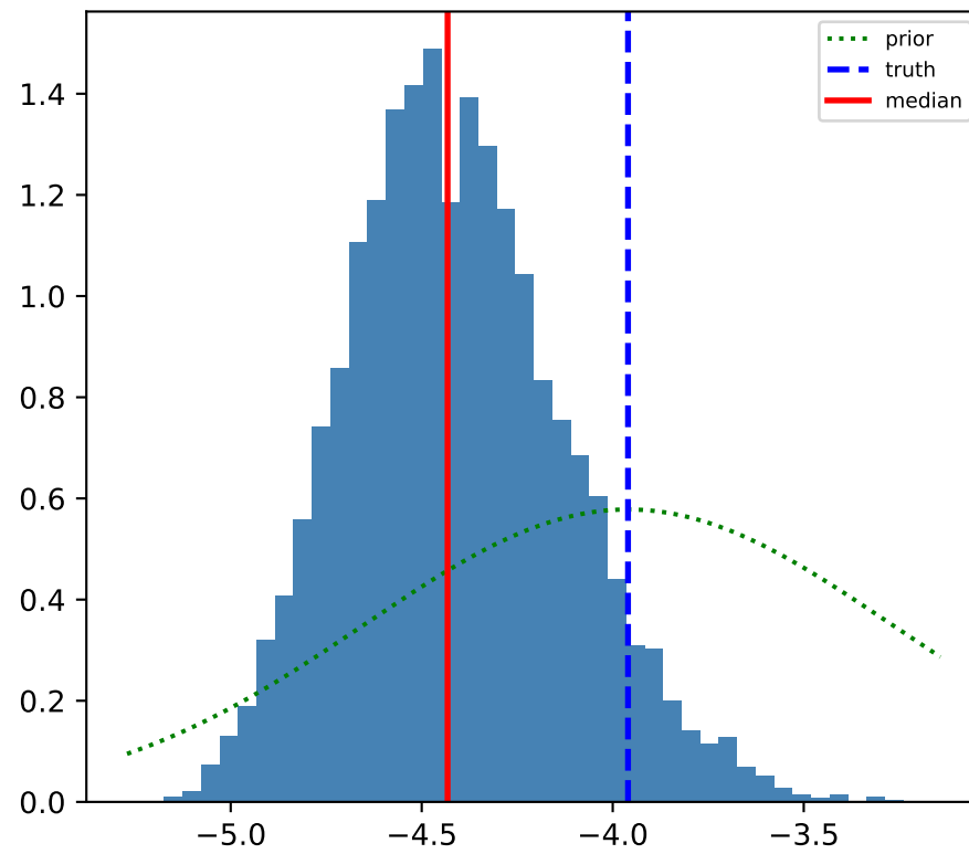
\log \phi_*
