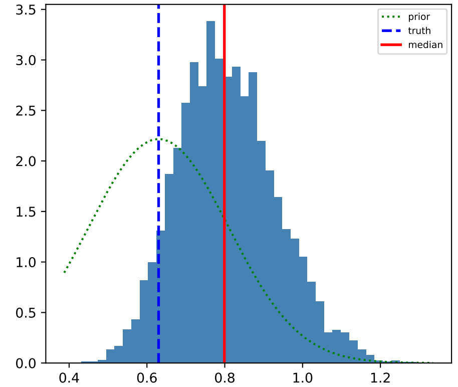
\beta
