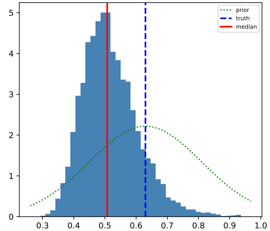
\beta
