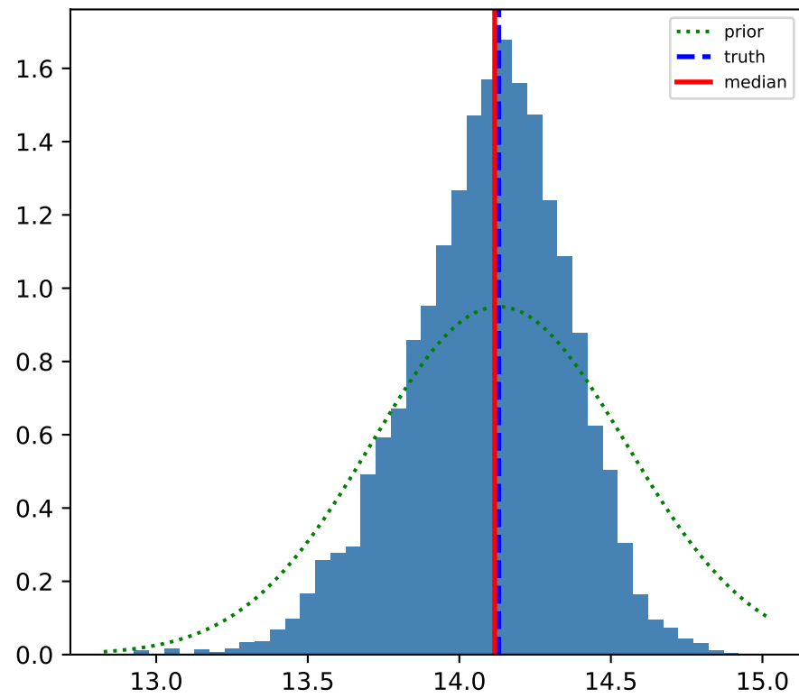
M_*
