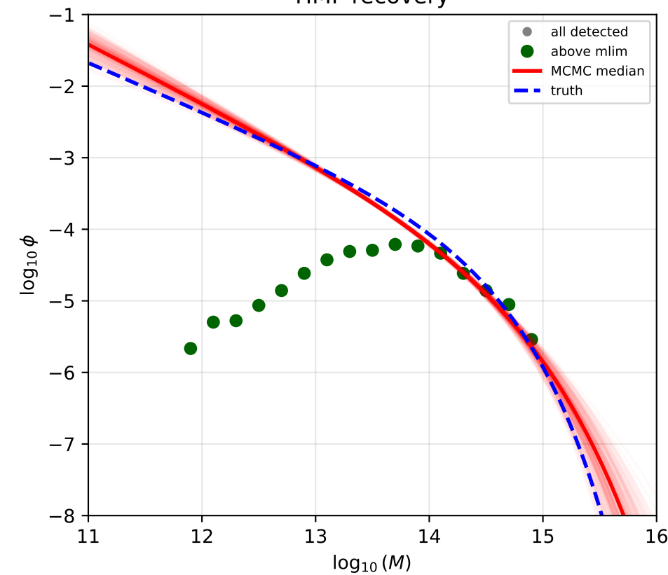
M_*
