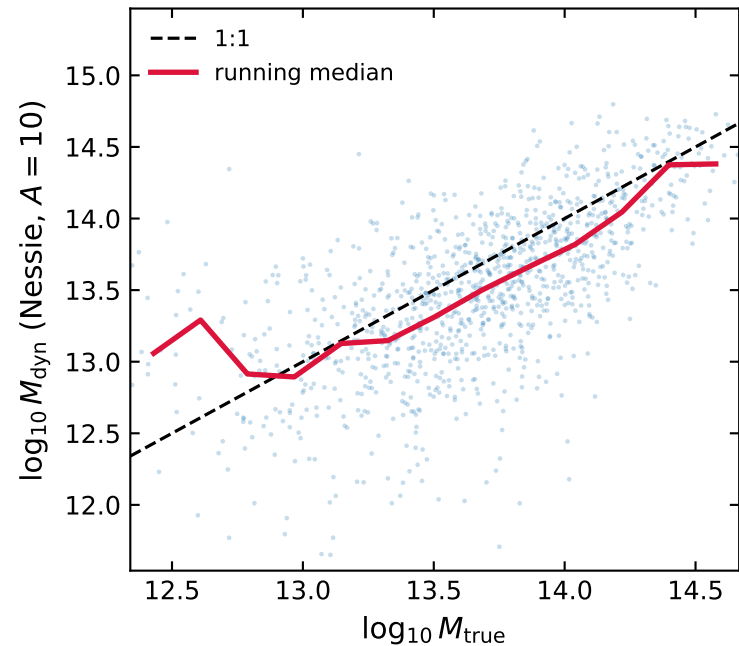
Recovered vs true mass
