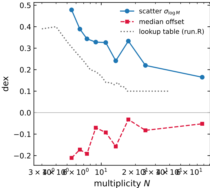
Mass error model
