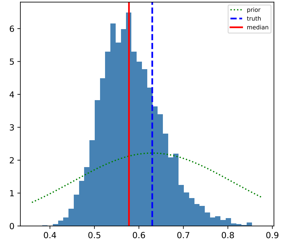
\beta
