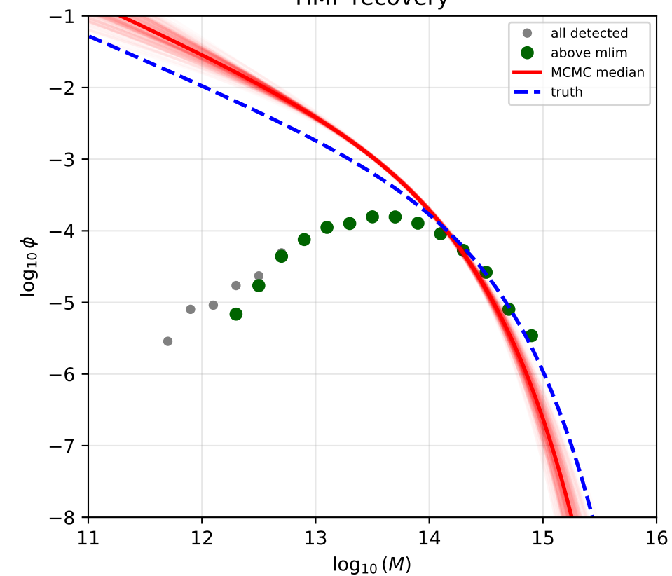
M_*
