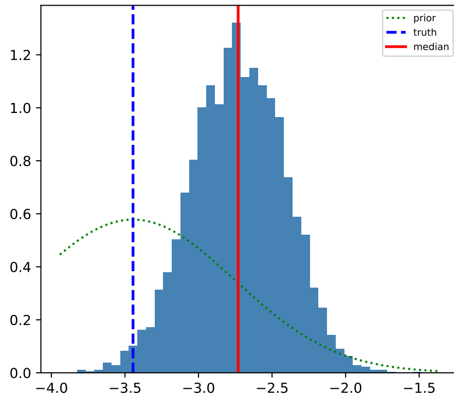
\log \phi_*
