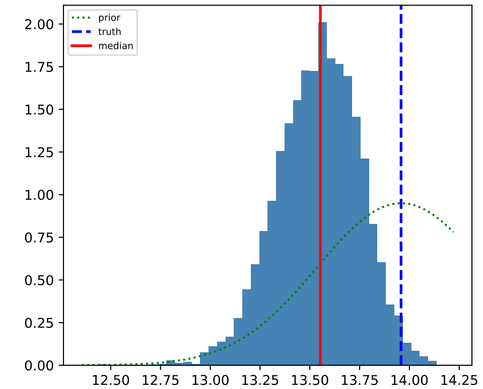
M_*
