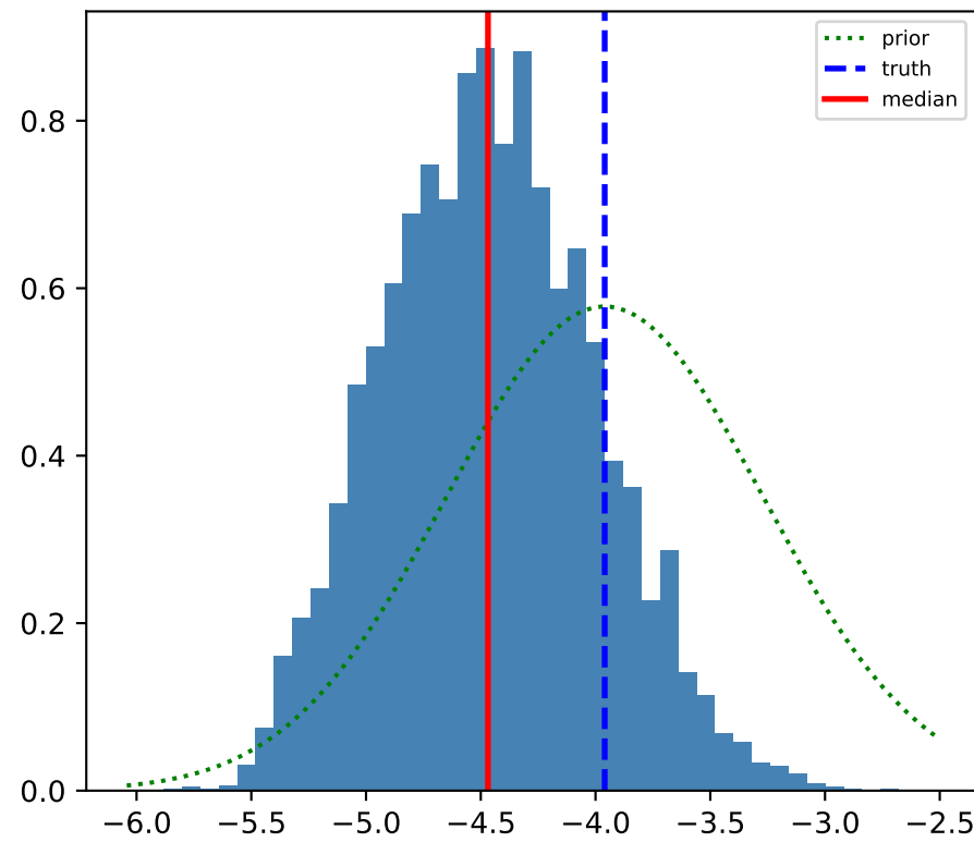
\log \phi_*
