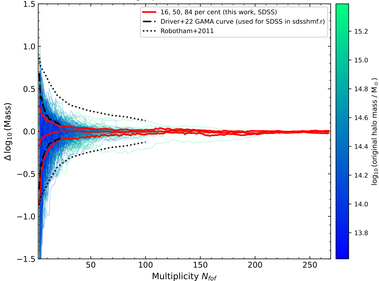
Nessie SDSS, groups with N > 20 , faintest-first removal
