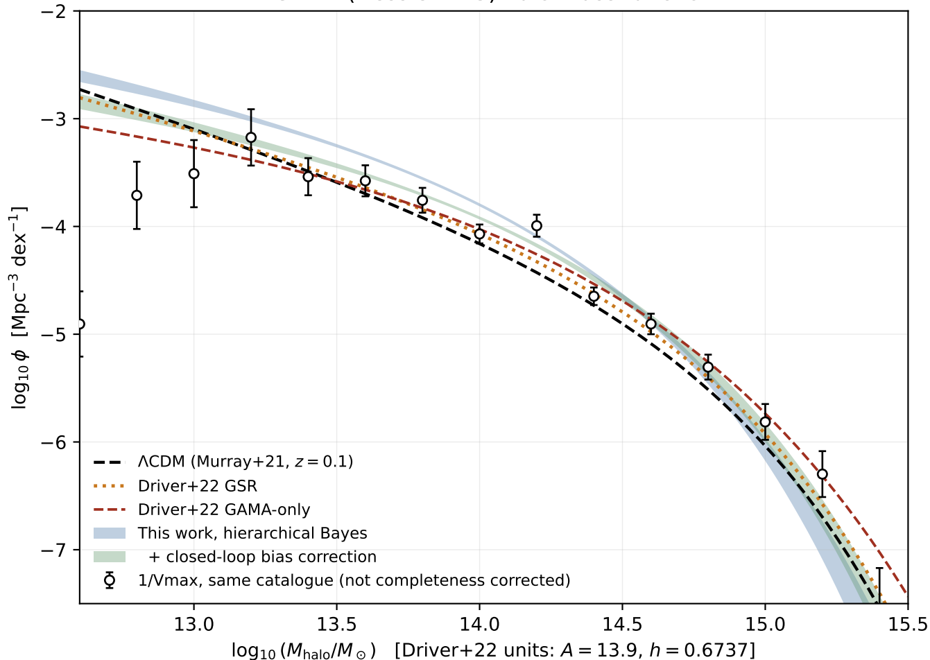
GAMA (Nessie DMU) halo mass function
