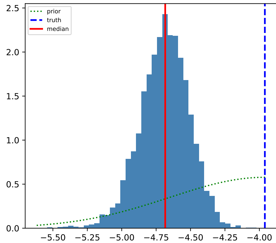
\log \phi_*
