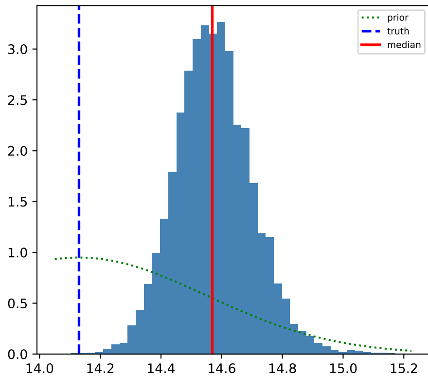
M_*
