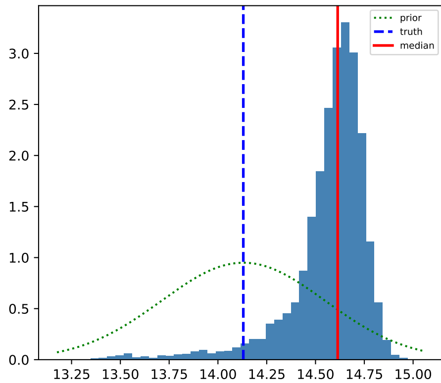
M_*
