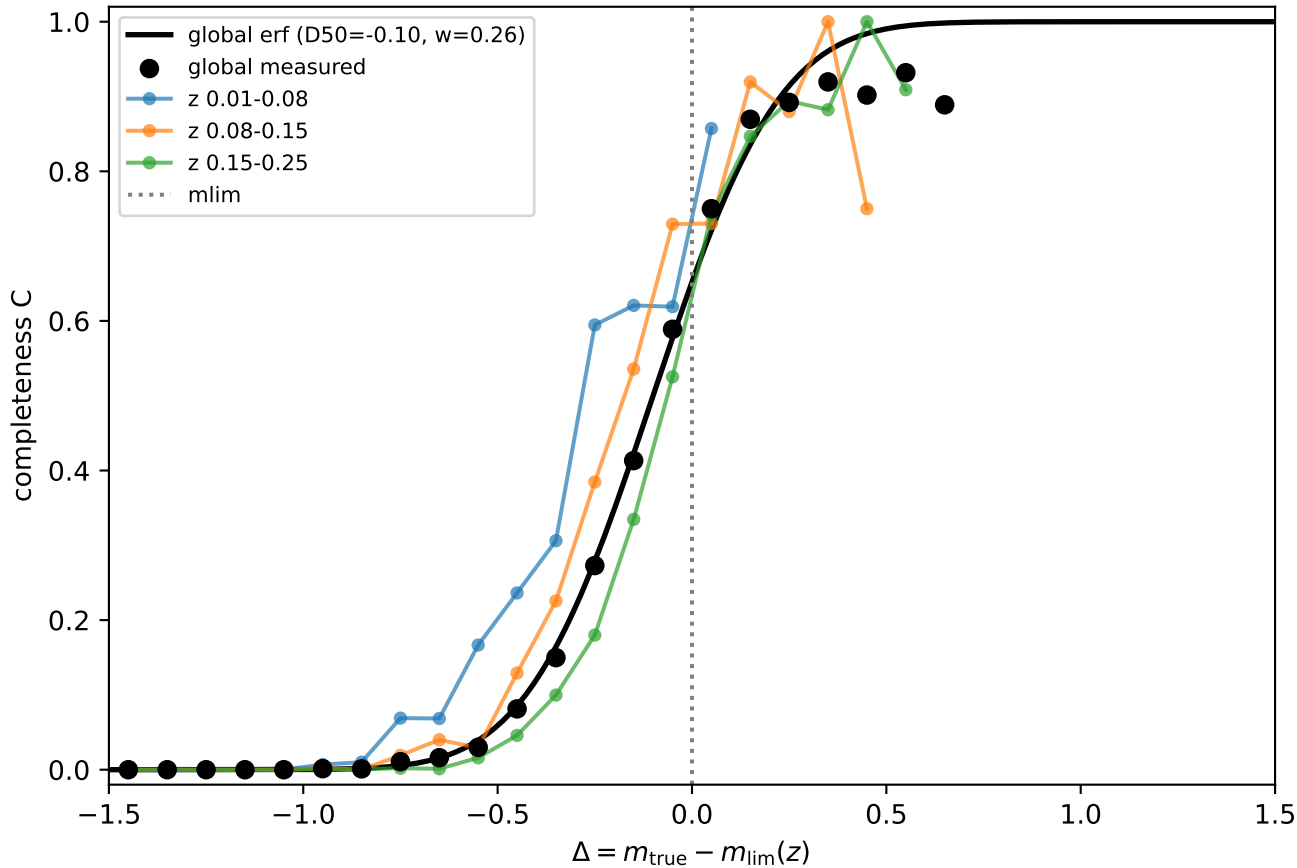
Mock completeness ramp
