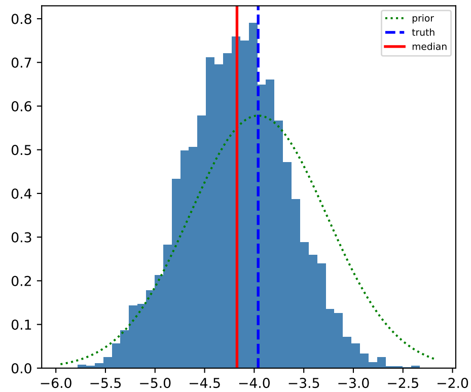
\log \phi_*
