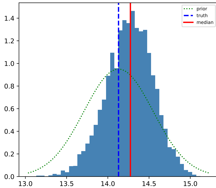
M_*
