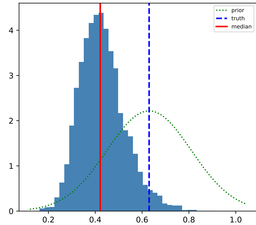
\beta
