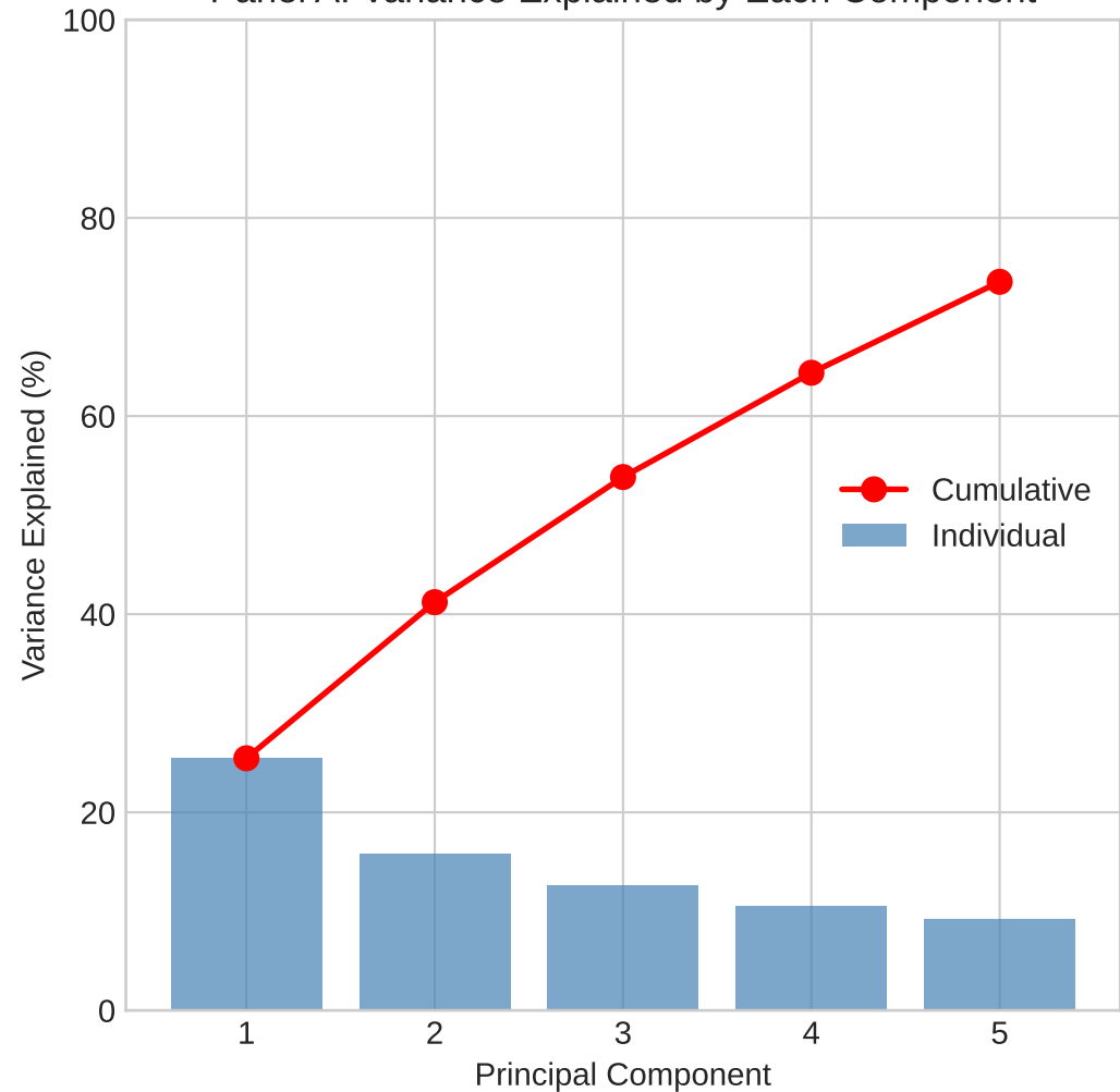
Panel A: Variance Explained by Each Component
