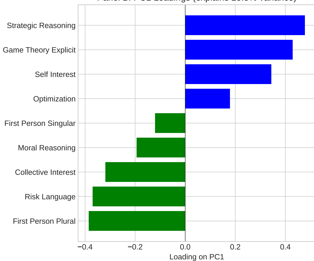
Panel B: PC1 Loadings (explains 25.5% variance)
