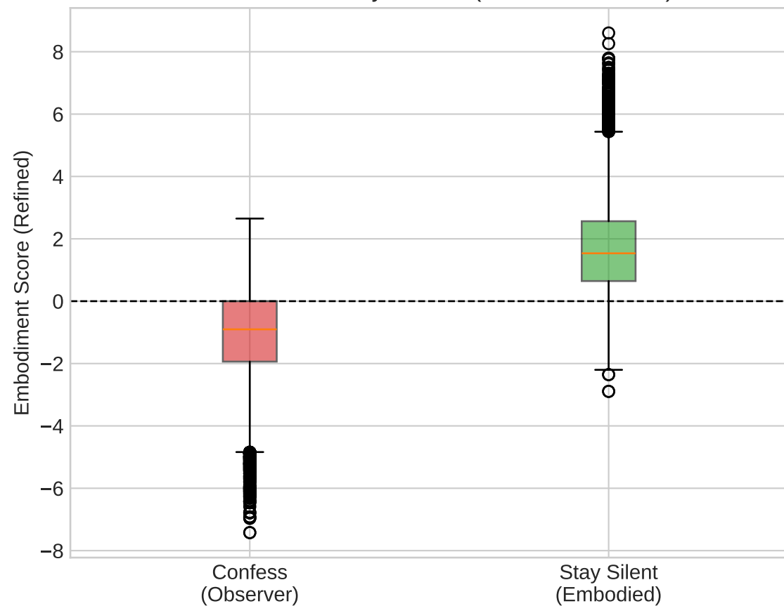
B: Embodiment by Choice (Cohen's d = 1.98 )
