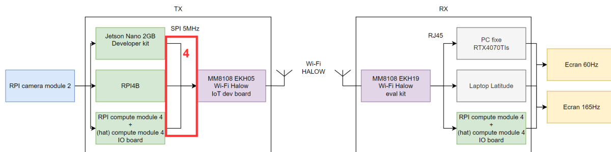
FIGURE 8 – (4) Interfaçage SPI
