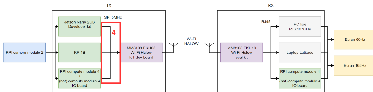
FIGURE 6 – (4) Interfaçage SPI
