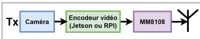
FIGURE 20 – Schéma Tx
