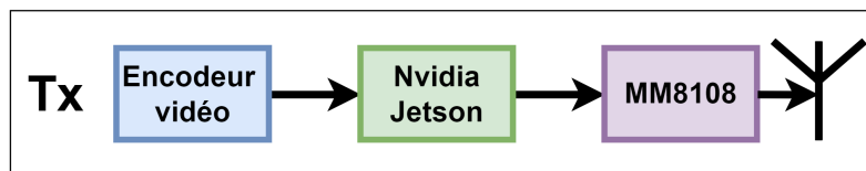
FIGURE 1 – Schéma Tx
