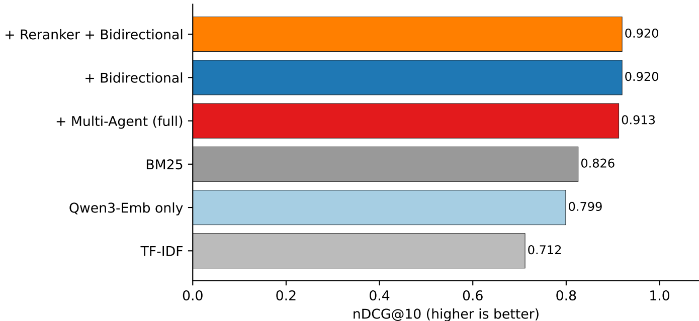
Ablation — nDCG@10 by configuration
