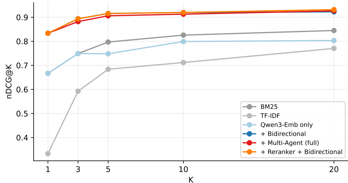
nDCG@K curves
