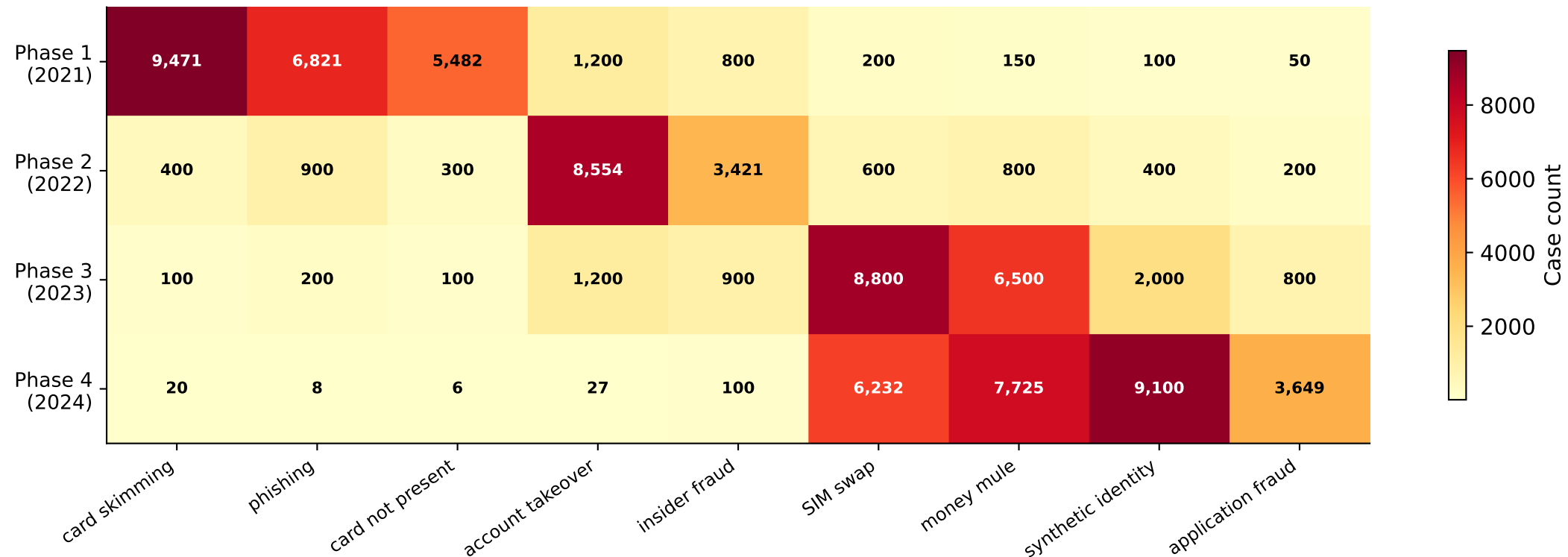
Fraud type evolution across phases — concept drift heatmap
