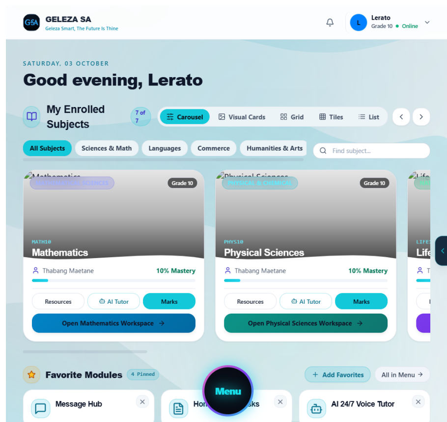
Figure 12. Learner Home — enrolled subjects carousel, Resources / AI Tutor / Marks shortcuts, and pinned Favorite Modules.
