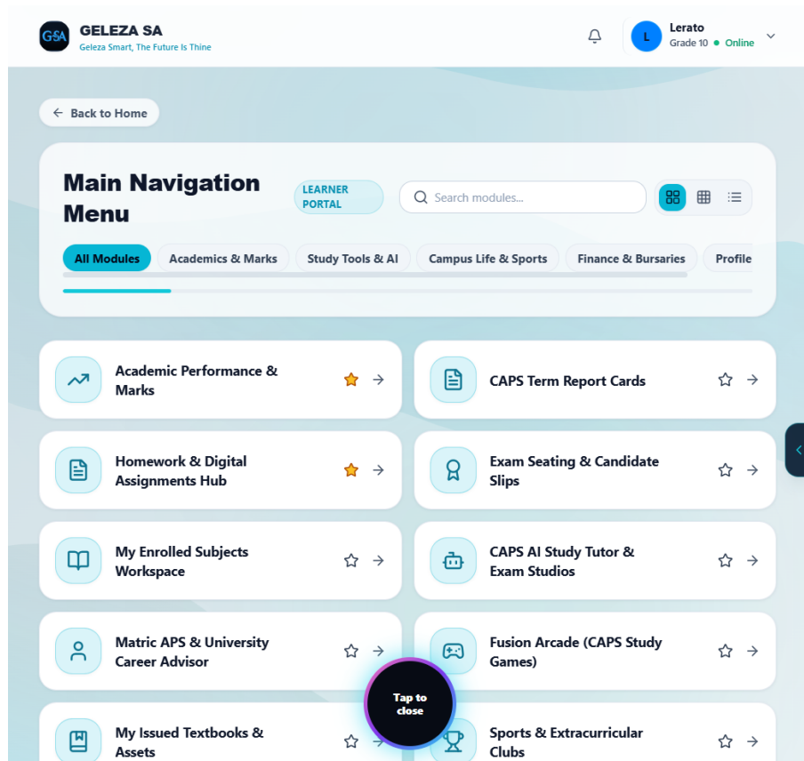
Figure 13. Learner Main Navigation Menu — academics, study/AI, campus life, finance, and profile modules.
