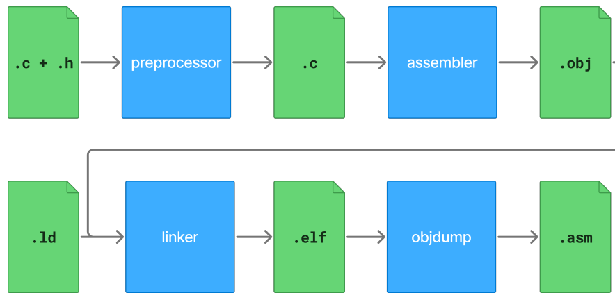
Figure 6: Diagram of the program build flow.
