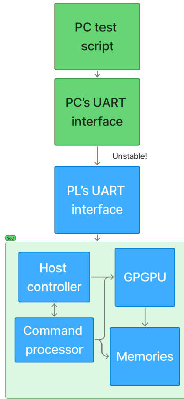
Figure 3: UART module in PL flow
