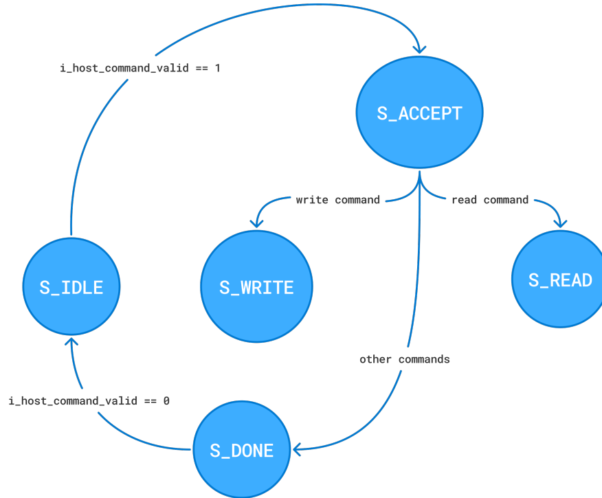
Figure 2: Host command processor FSM
