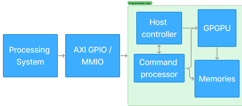
Figure 5: Flow of PS to PL communication
