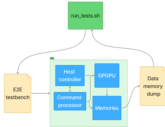
Figure 7: End-to-end testing flow
