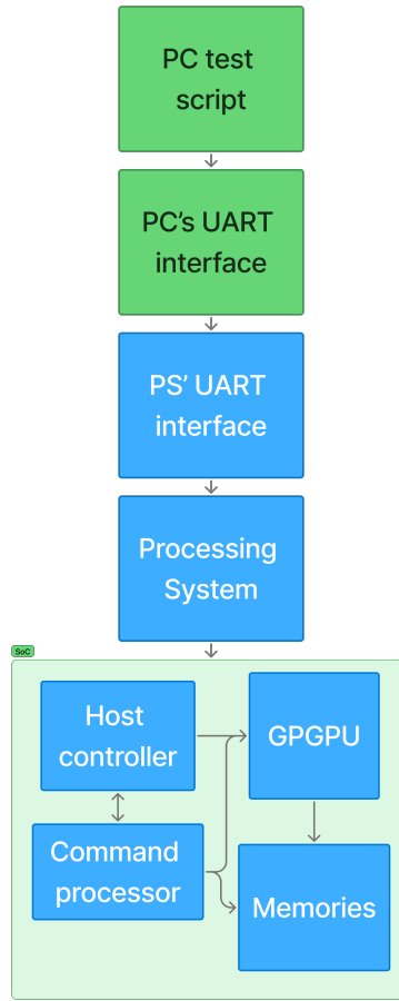
Figure 4: Revised architecture using PS for UART
