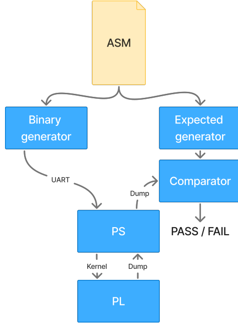
Figure 8: FPGA End-to-End test flow
