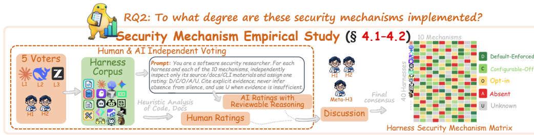
Figure 3: Security mechanism rating and consensus workflow in RQ2.
