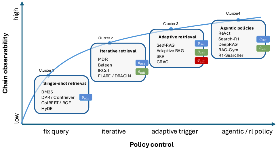
Fig. 4. Retrieval-based methods. As retrieval control shifts from fixed-query retrieval to iterative, adaptive, and agentic retrieval, the system can increase chain observability but must manage noise, cost, and query drift.
