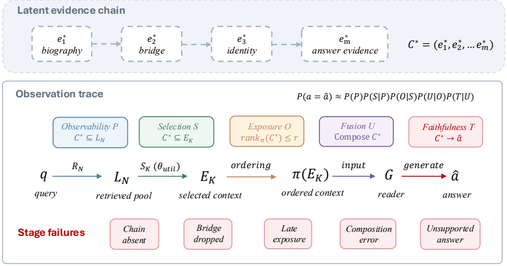
Fig. 1. Latent evidence-chain inference view of multi-hop RAG. The target object is an unobserved support chain C^* , while the system observes only a retrieved pool L_N , a budgeted context E_K , an ordering \pi(E_K) , and a generated answer \hat{a} . The five estimands diagnose where the chain becomes absent, dropped, poorly exposed, incorrectly fused, or used only post hoc rather than causally.
