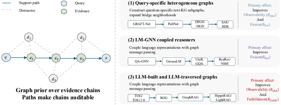
Fig. 3. Graph-based methods as chain-structure estimators. Graph methods improve chain observability by expanding local neighborhoods, constrain fusion through structured paths, and improve faithfulness when paths or subgraphs can be audited.
