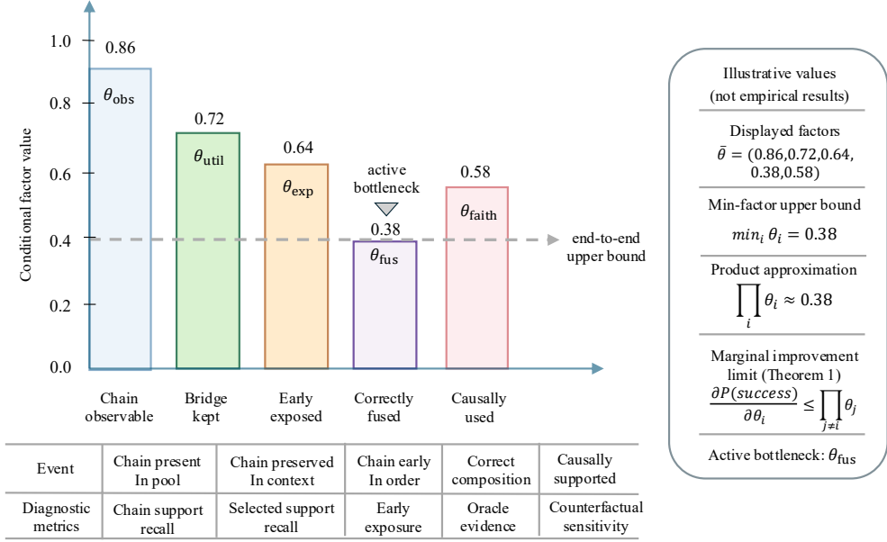
Fig. 2. Bottleneck visualization of the five estimands. End-to-end success is upper-bounded by the weakest factor across observability, utility, exposure, fusion, and faithfulness.
