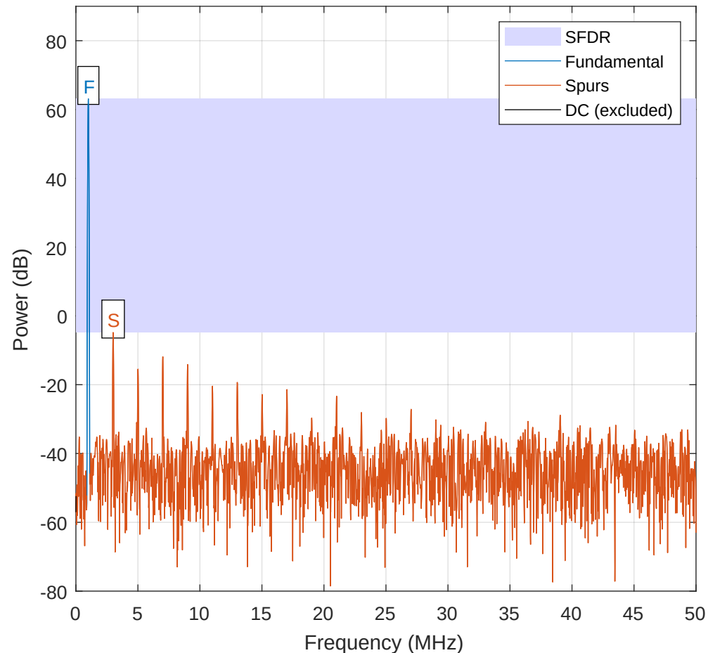
Spectre Sortie Chisel (Materiel)
