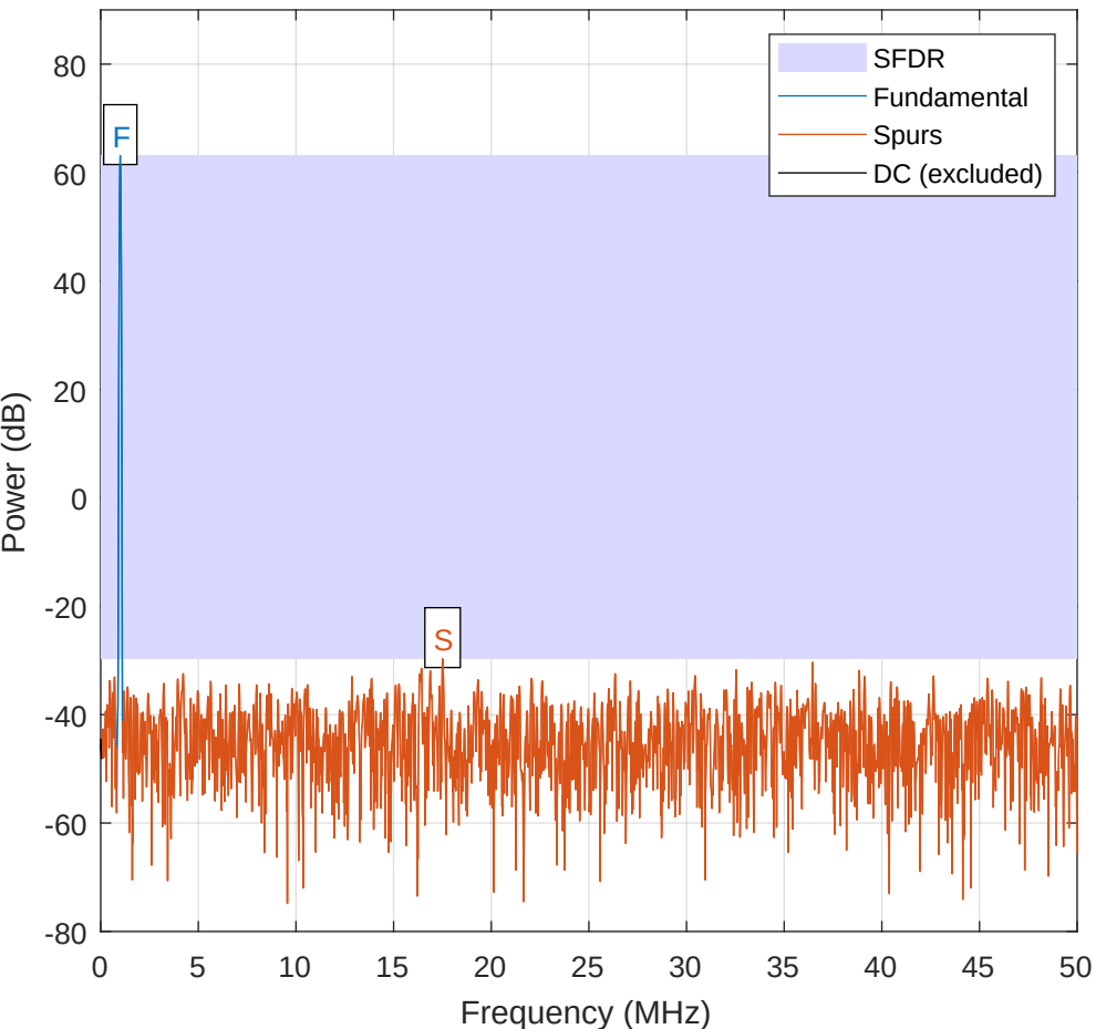
Spectre Reference LUT (MATLAB)
