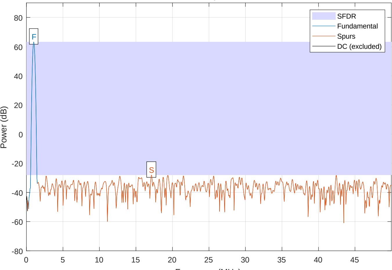
Chisel Output Spectrum SFDR = 90.72 dBc | SNR = 73.96 dB
