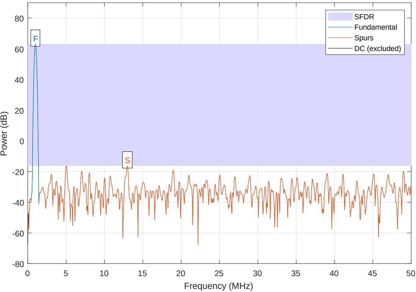
Chisel Output Spectrum SFDR = 78.71 dBc | SNR = 68.75 dB
