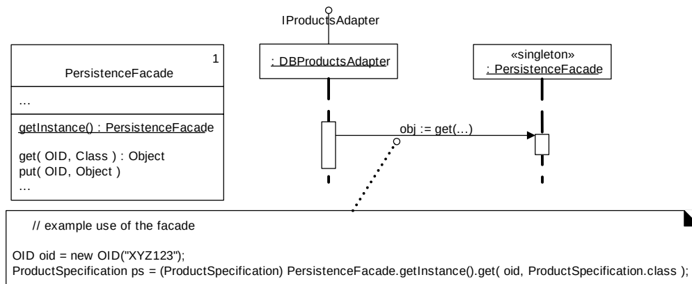
Figure 34.4 The PersistenceFacade.
