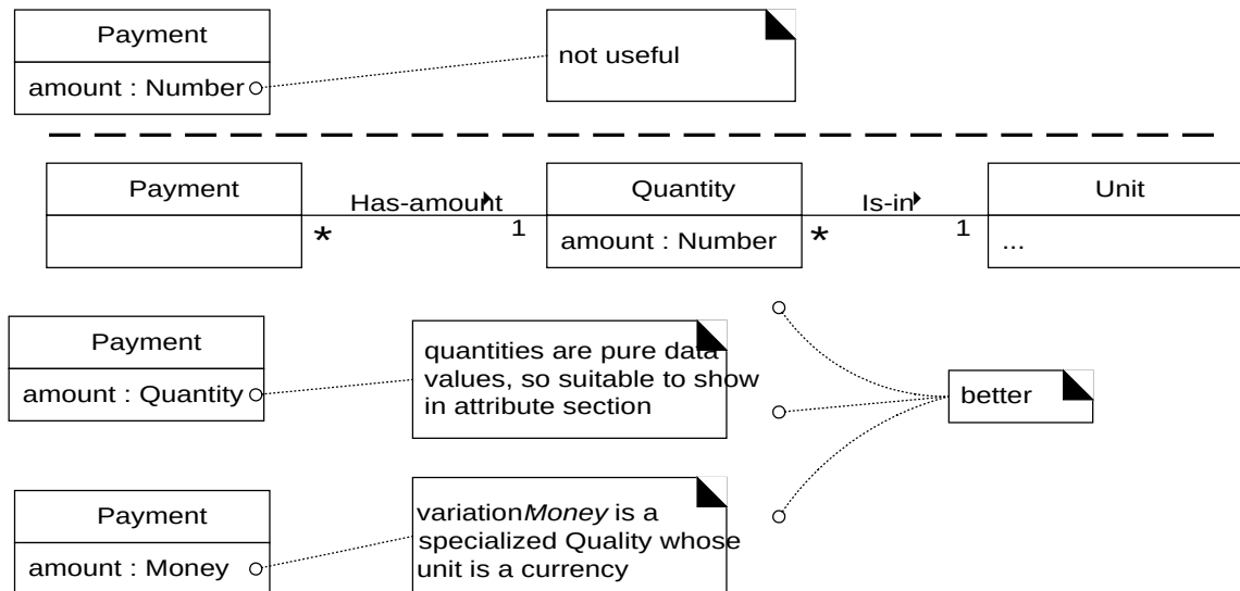
Figure 12.6 Modeling quantities.
