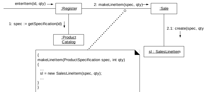
Figure 18.3 Parameter visibility.
