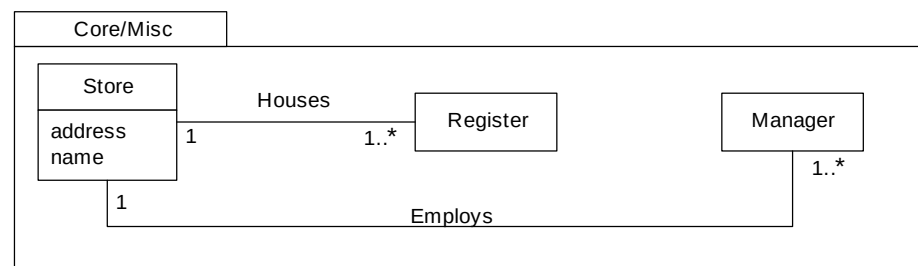
Figure 27.22 Core package.
