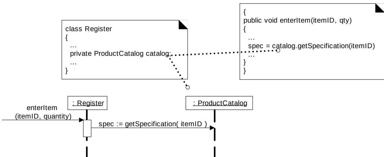
Figure 18.2 Attribute visibility.
