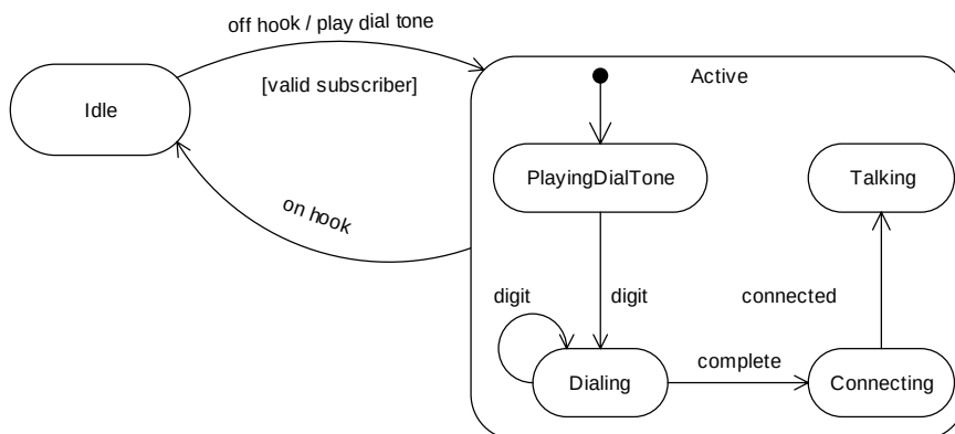
Figure 29.5 Nested states.
