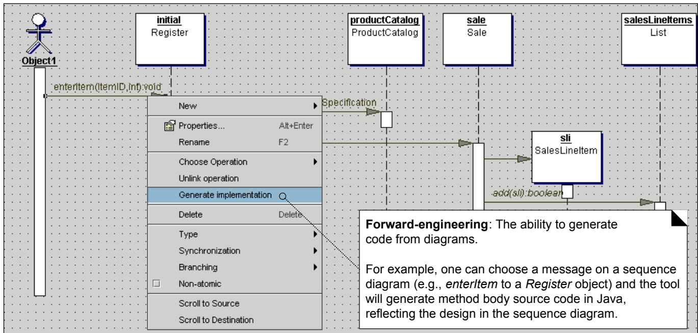
Figure 35.1 Forward-engineering.
