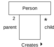
Figure 27.15 Reflexive association.
