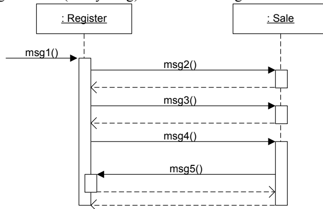
Figure 15.18 Showing returns.
