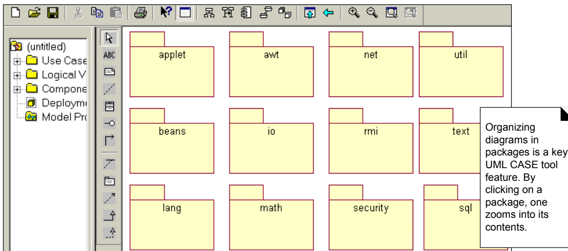
Figure 35.4 Managing packages.
