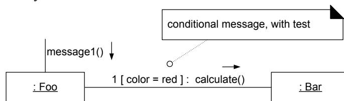
Figure 15.12 Conditional message.
