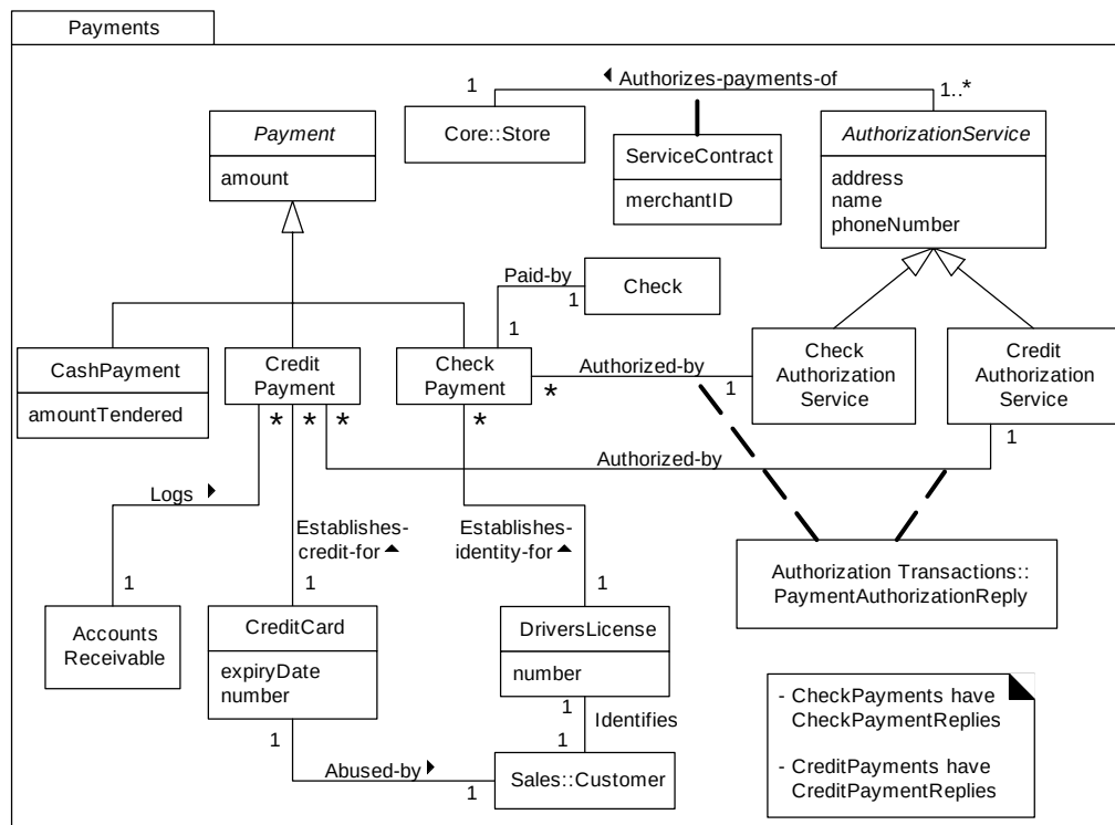
Figure 27.23 Payments package.
