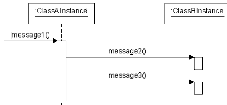
Figure 15.2 Sequence diagram.
