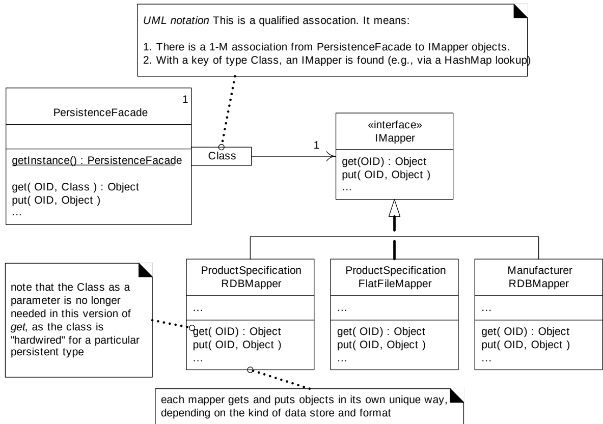
Figure 34.5 Database Mappers.
