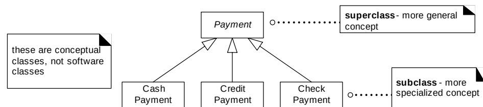
Figure 26.1 Generalization-specialization hierarchy.
