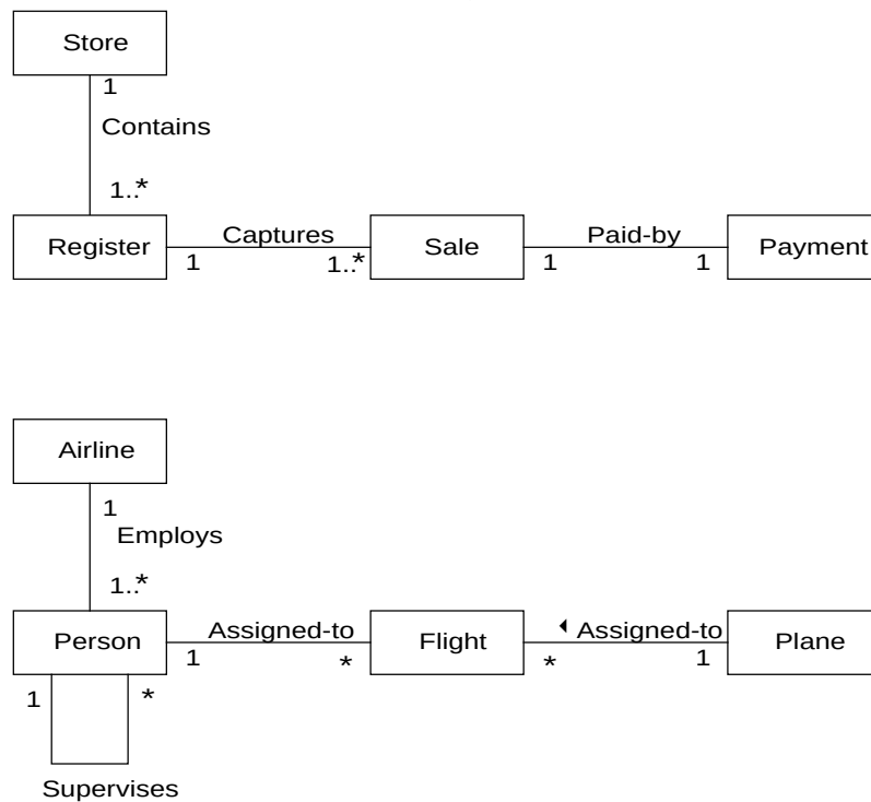
Figure 11.6 Association names.
