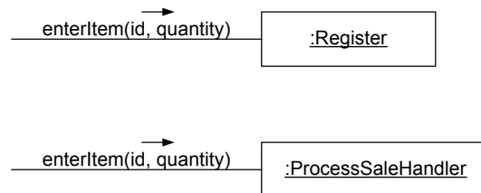
Figure 16.15 Controller choices.
