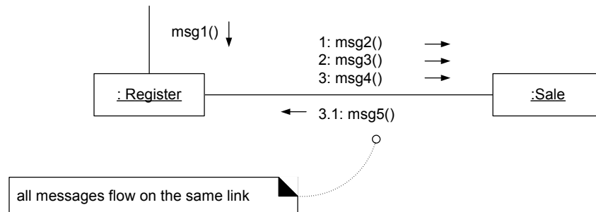
Figure 15.7 Messages.
