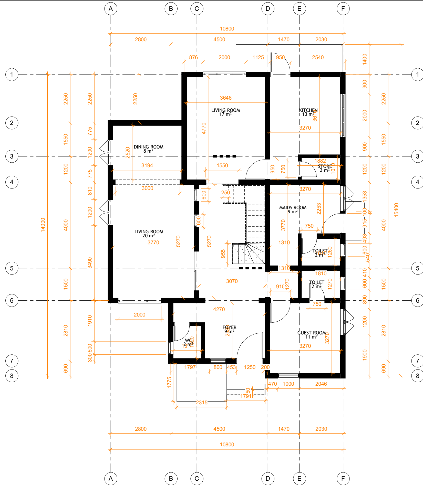
1 GROUND FLOOR PLAN 1 : 45
