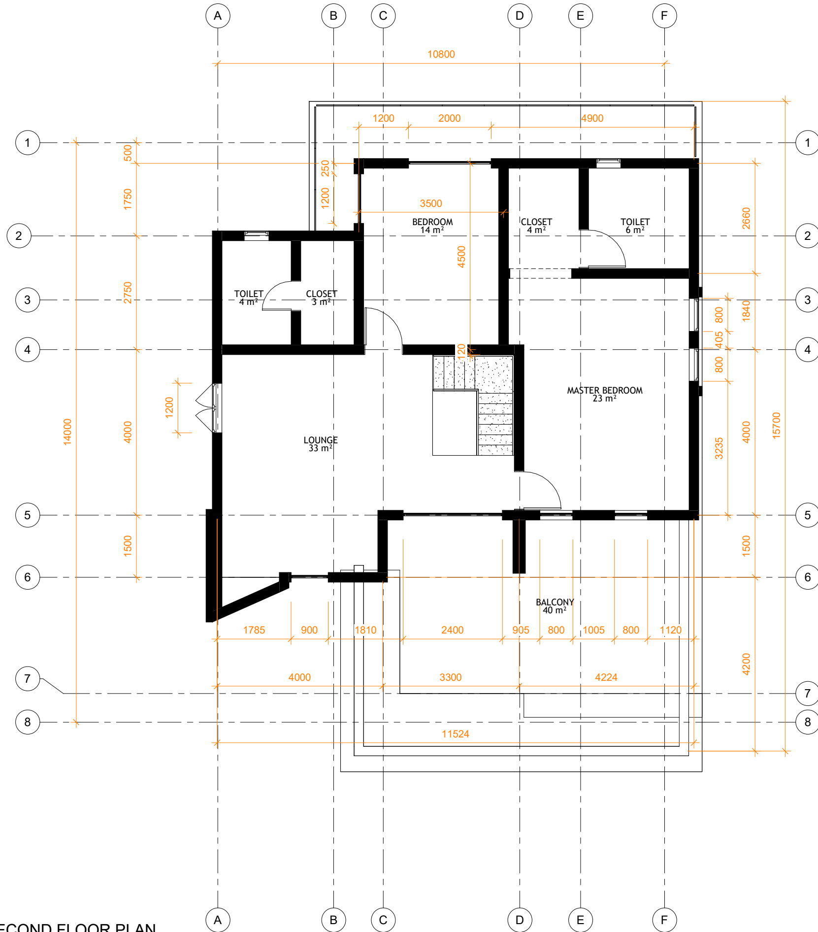
1 SECOND FLOOR PLAN 1 : 45
