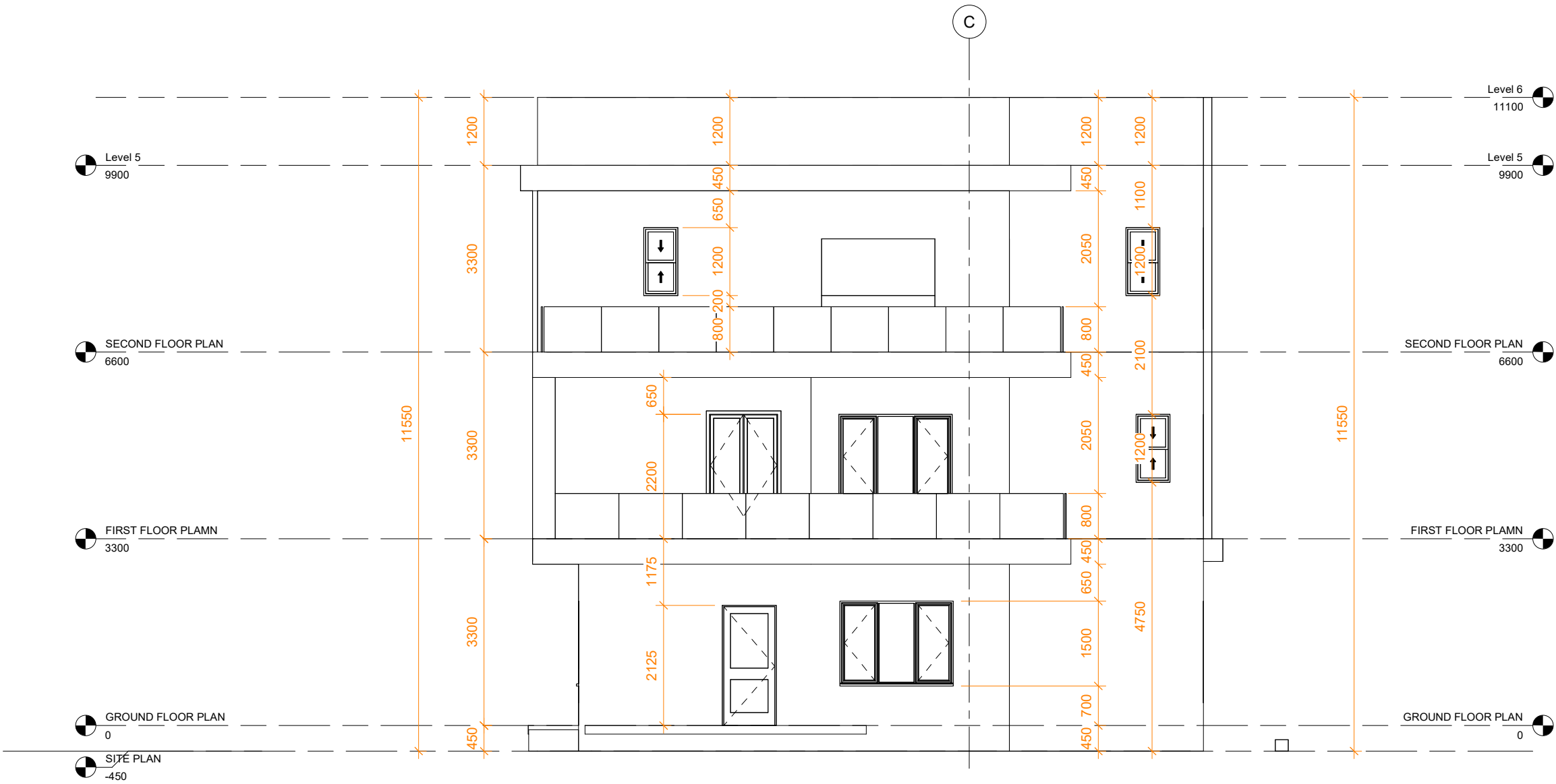
1 BACK ELEVATION 1 : 45
