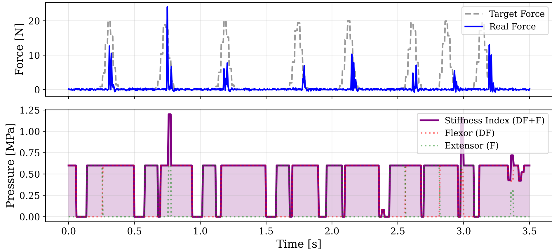
Zero-shot Adaptation to Unseen Groove (Extreme 170 BPM)
