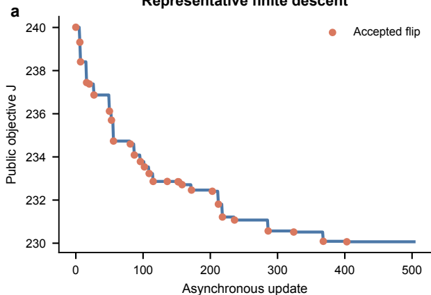
Representative finite descent
