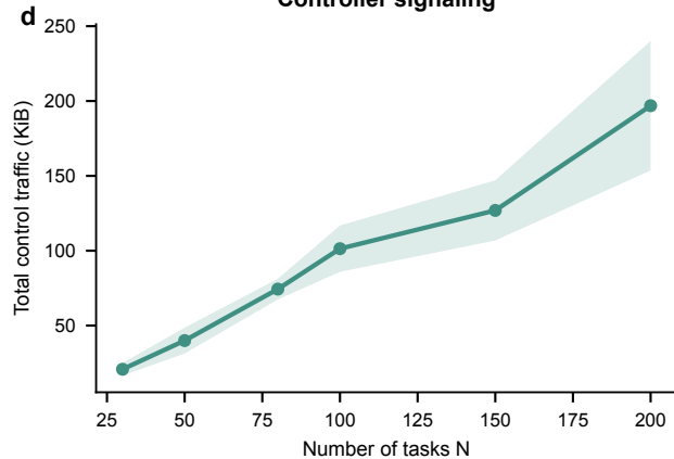
Controller signaling
