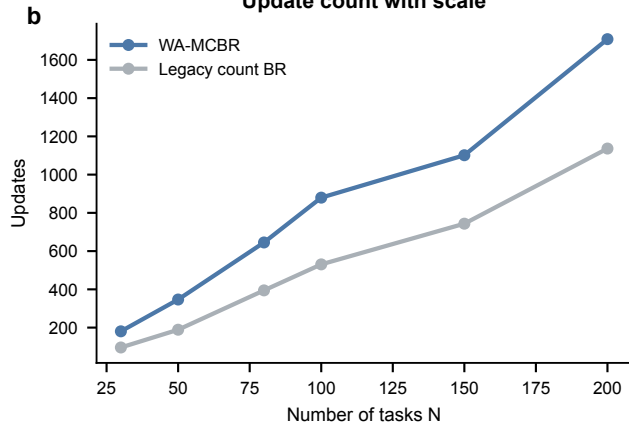
Update count with scale
