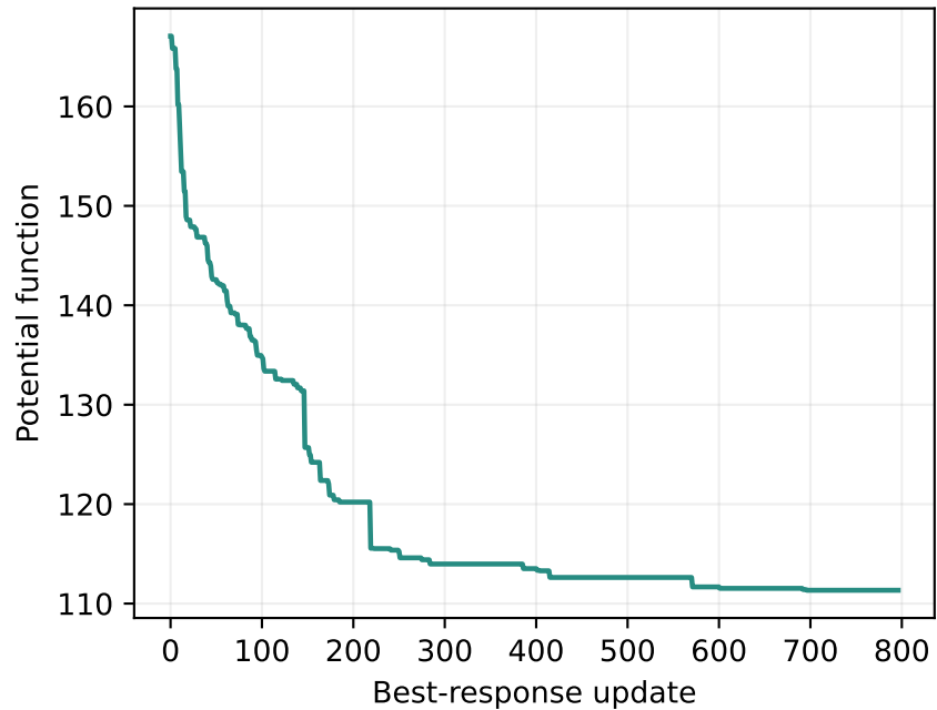
B Potential descent
