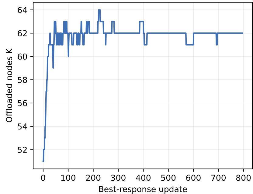
A Strategy convergence
